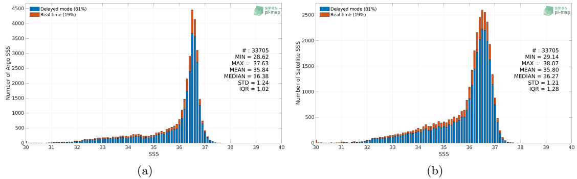
Figure 2: Histograms of SSS from Argo (a) and SMOS SSS L3 v8 - 9 Days (CATDS-CECOS-LOCEAN) (b) considering all match-up pairs per bins of 0.1 over the Gulf Stream Pi-MEP region and for the full satellite product period.
