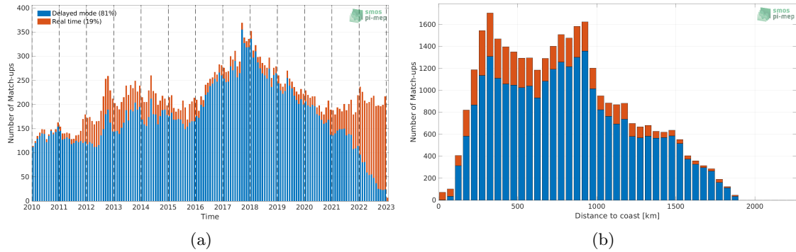
Figure 1: Number of match-ups between Argo and SMOS SSS L3 v8 - 9 Days (CATDS-CECOS-LOCEAN) SSS as a function of time (a) and as function of the distance to coast (b) over the Gulf Stream Pi-MEP region and for the full satellite product period.
