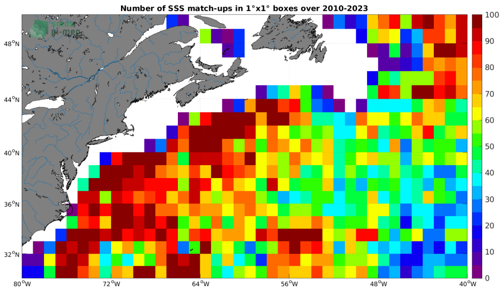
Figure 4: Number of SSS match-ups between Argo SSS and the SMOS SSS L3 v8 - 9 Days (CATDS-CECOS-LOCEAN) SSS product for the Gulf Stream Pi-MEP region over 1^\circ \times 1^\circ boxes and for the full satellite product period.
