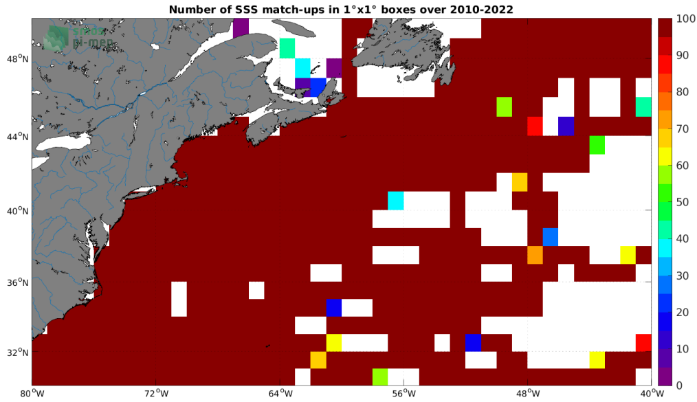
Figure 4: Number of SSS match-ups between TSG (SAMOS) SSS and the SMOS SSS L3 v8 - 18 Days (CATDS-CECOS-LOCEAN) SSS product for the Gulf Stream Pi-MEP region over 1^\circ \times 1^\circ boxes and for the full satellite product period.
