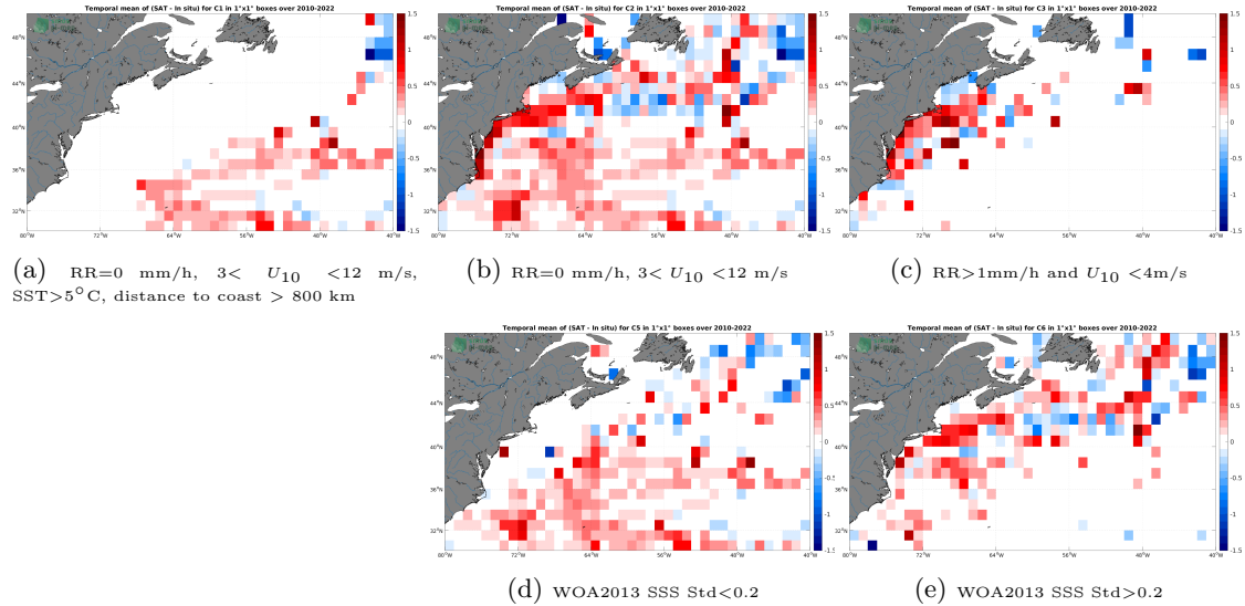
Figure 12: Temporal mean gridded over spatial boxes of size 1^{\circ}\times 1^{\circ} of \Delta\text{SSS} (SMOS SSS L3 v8 - 18 Days (CATDS-CECOS-LOCEAN) - TSG (SAMOS)) for 5 different subdatasets corresponding to:RR=0 mm/h, 3 < U_{10} < 12 m/s, SST >5^{\circ}\text{C} , distance to coast > 800 km (a), RR=0 mm/h, 3 < U_{10} < 12 m/s (b), RR >1 mm/h and U_{10} < 4 m/s (c), WOA2013 SSS Std <0.2 (d), WOA2013 SSS Std >0.2 (e).
