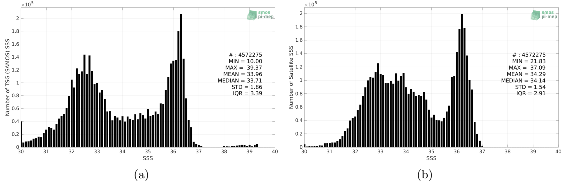
Figure 2: Histograms of SSS from TSG (SAMOS) (a) and SMOS SSS L3 v8 - 18 Days (CATDS-CECOS-LOCEAN) (b) considering all match-up pairs per bins of 0.1 over the Gulf Stream Pi-MEP region and for the full satellite product period.
