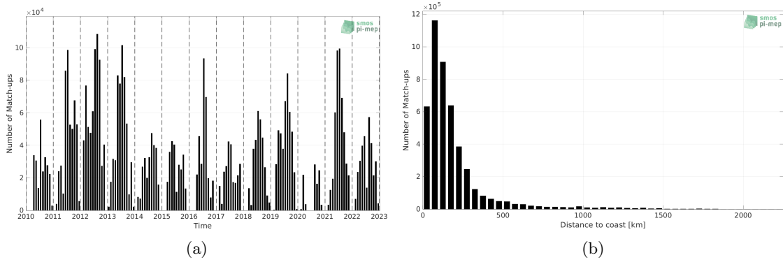
Figure 1: Number of match-ups between TSG (SAMOS) and SMOS SSS L3 v8 - 18 Days (CATDS-CECOS-LOCEAN) SSS as a function of time (a) and as function of the distance to coast (b) over the Gulf Stream Pi-MEP region and for the full satellite product period.
