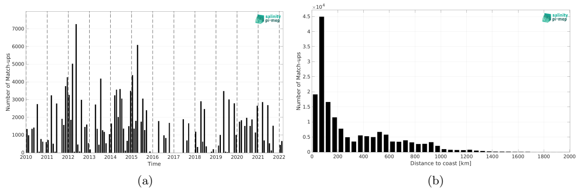
Figure 1: Number of match-ups between TSG (LEGOS-DM) and SMOS SSS L3 v8 - 18 Days (CATDS-CEC-LOCEAN) SSS as a function of time (a) and as function of the distance to coast (b) over the Gulf Stream Pi-MEP region and for the full satellite product period.
