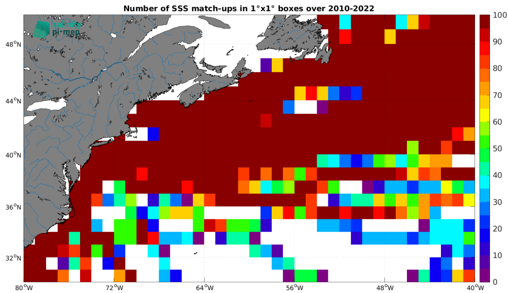
Figure 4: Number of SSS match-ups between TSG (LEGOS-DM) SSS and the SMOS SSS L3 v8 - 18 Days (CATDS-CEC-LOCEAN) SSS product for the Gulf Stream Pi-MEP region over 1^\circ \times 1^\circ boxes and for the full satellite product period.
