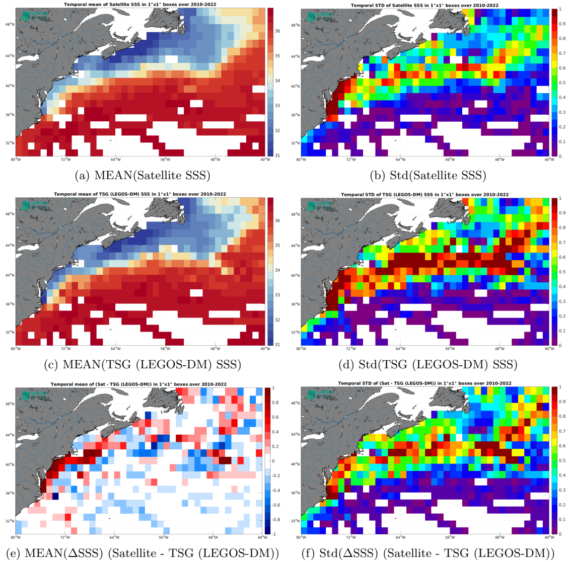
Figure 6: Temporal mean (left) and Std (right) of SSS from SMOS SSS L3 v8 - 18 Days (CATDS-CEC-LOCEAN) (top), TSG (LEGOS-DM) (middle), and of \Delta SSS (Satellite - TSG (LEGOS-DM)). Only match-up pairs are used to generate these maps.
