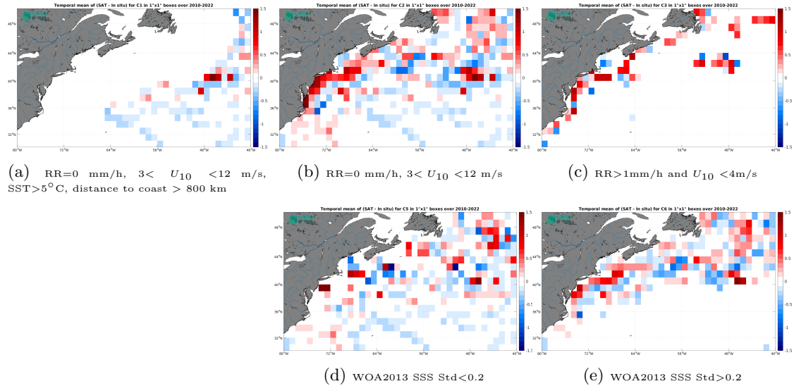
Figure 12: Temporal mean gridded over spatial boxes of size 1^{\circ}\times 1^{\circ} of \Delta\text{SSS} (SMOS SSS L3 v8 - 18 Days (CATDS-CEC-LOCEAN) - TSG (LEGOS-DM)) for 5 different subdatasets corresponding to:RR=0 mm/h, 3 < U_{10} < 12 m/s, SST >5^{\circ}\text{C} , distance to coast > 800 km (a), RR=0 mm/h, 3 < U_{10} < 12 m/s (b), RR >1 mm/h and U_{10} < 4 m/s (c), WOA2013 SSS Std <0.2 (d), WOA2013 SSS Std >0.2 (e).
