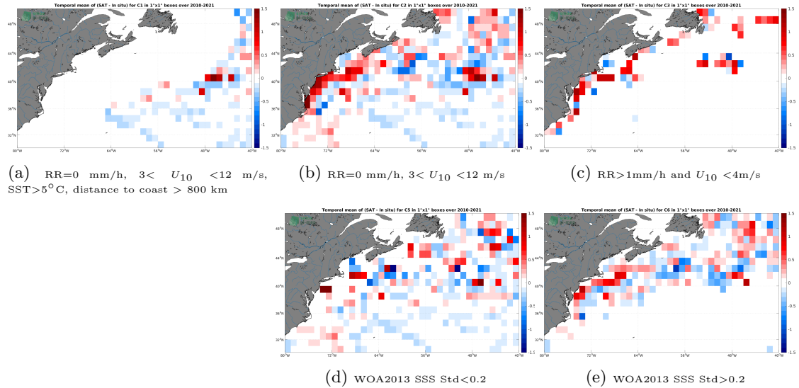
Figure 12: Temporal mean gridded over spatial boxes of size 1^{\circ}\times 1^{\circ} of \Delta\text{SSS} (SMOS SSS L3 v8 - 18 Days (CATDS-CECOS-LOCEAN) - TSG (LEGOS-DM)) for 5 different subdatasets corresponding to:RR=0 mm/h, 3 < U_{10} < 12 m/s, SST >5^{\circ}\text{C} , distance to coast > 800 km (a), RR=0 mm/h, 3 < U_{10} < 12 m/s (b), RR >1 mm/h and U_{10} < 4 m/s (c), WOA2013 SSS Std <0.2 (d), WOA2013 SSS Std >0.2 (e).
