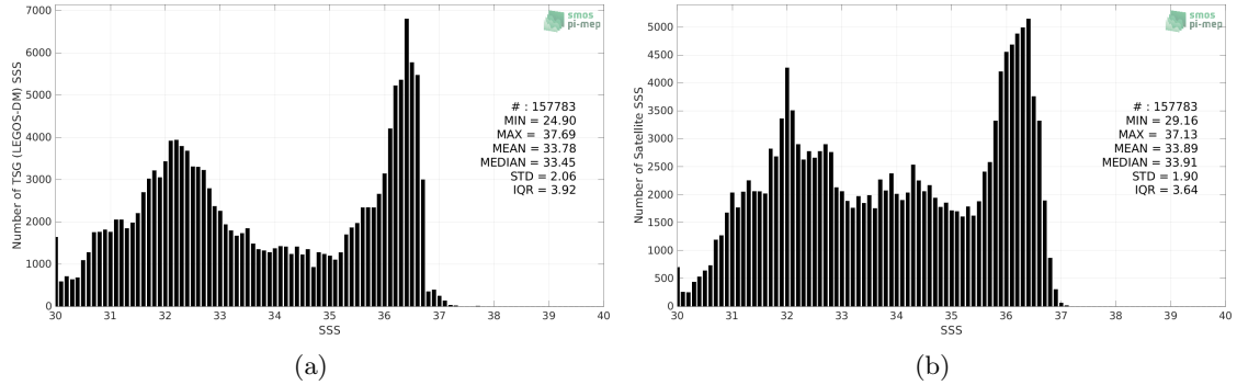
Figure 2: Histograms of SSS from TSG (LEGOS-DM) (a) and SMOS SSS L3 v8 - 18 Days (CATDS-CECOS-LOCEAN) (b) considering all match-up pairs per bins of 0.1 over the Gulf Stream Pi-MEP region and for the full satellite product period.
