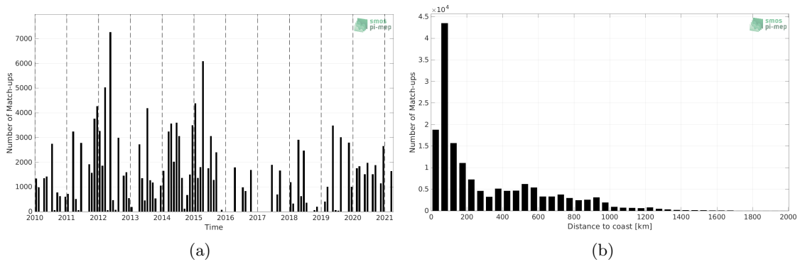
Figure 1: Number of match-ups between TSG (LEGOS-DM) and SMOS SSS L3 v8 - 18 Days (CATDS-CECOS-LOCEAN) SSS as a function of time (a) and as function of the distance to coast (b) over the Gulf Stream Pi-MEP region and for the full satellite product period.
