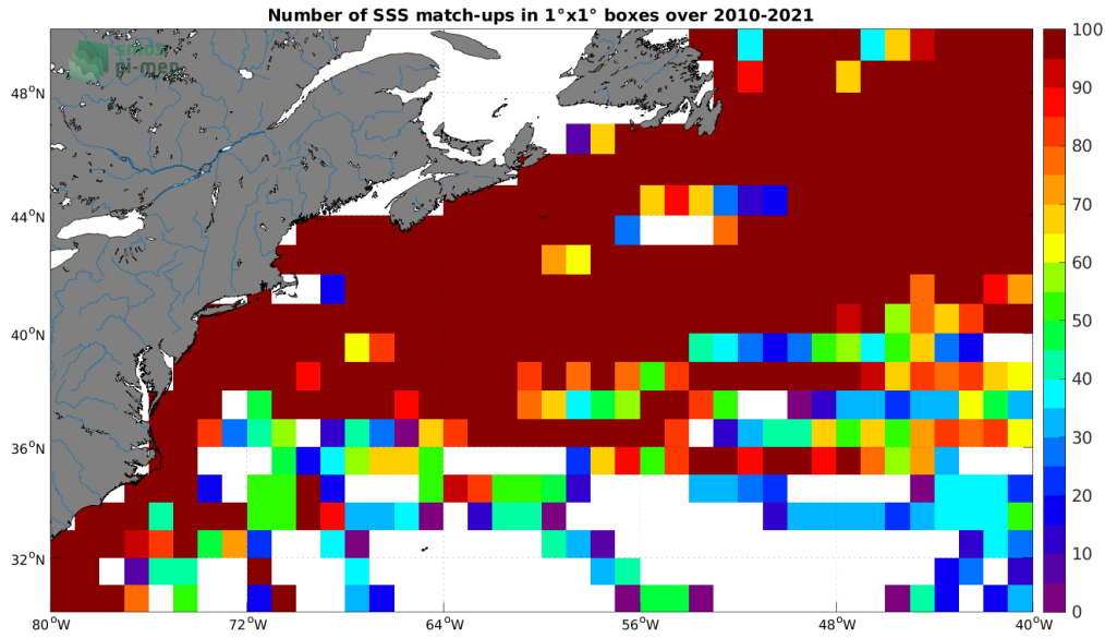
Figure 4: Number of SSS match-ups between TSG (LEGOS-DM) SSS and the SMOS SSS L3 v8 - 18 Days (CATDS-CECOS-LOCEAN) SSS product for the Gulf Stream Pi-MEP region over 1^\circ \times 1^\circ boxes and for the full satellite product period.
