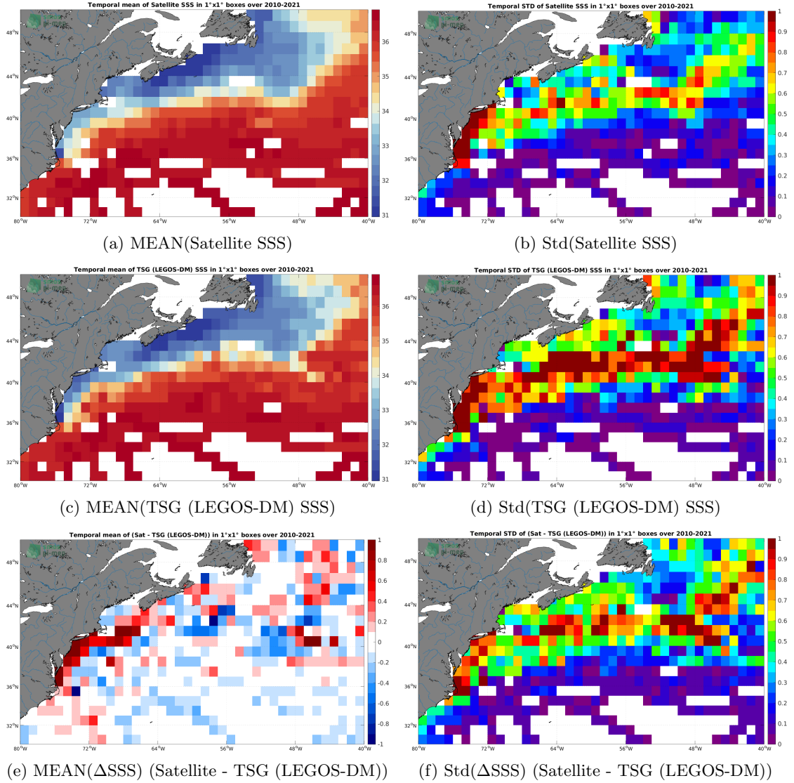
Figure 6: Temporal mean (left) and Std (right) of SSS from SMOS SSS L3 v8 - 18 Days (CATDS-CECOS-LOCEAN) (top), TSG (LEGOS-DM) (middle), and of \Delta SSS (Satellite - TSG (LEGOS-DM)). Only match-up pairs are used to generate these maps.
