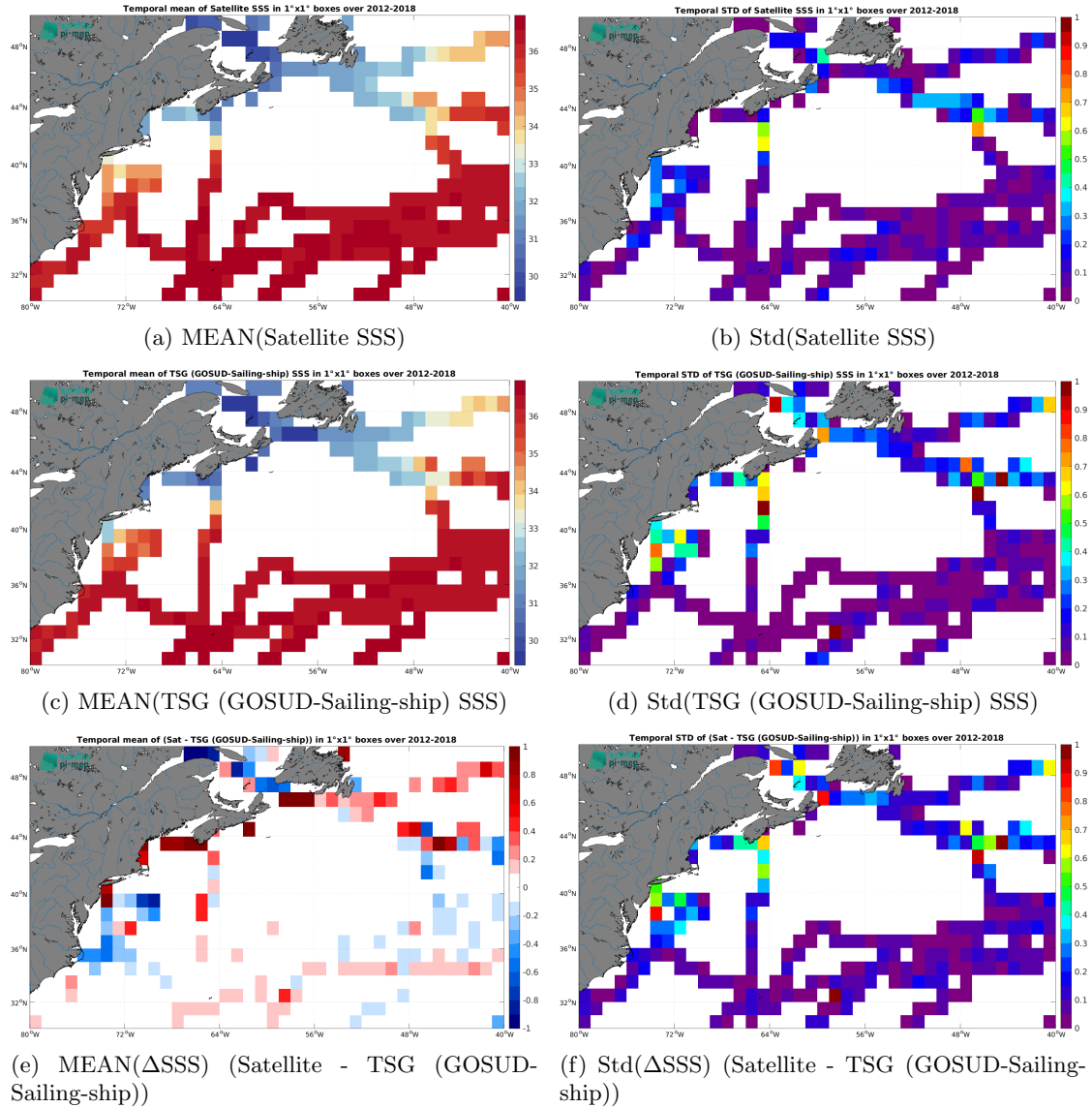
Figure 6: Temporal mean (left) and Std (right) of SSS from SMOS SSS L3 v8 - 18 Days (CATDS-CEC-LOCEAN) (top), TSG (GOSUD-Sailing-ship) (middle), and of \Delta SSS (Satellite - TSG (GOSUD-Sailing-ship)). Only match-up pairs are used to generate these maps.
