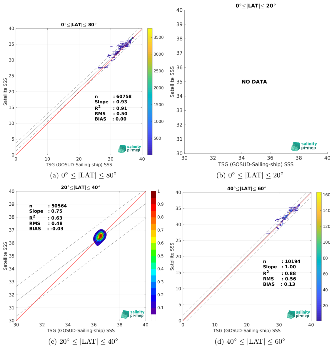
Figure 9: Contour maps of the concentration of SMOS SSS L3 v8 - 18 Days (CATDS-CEC-LOCEAN) SSS (y-axis) versus TSG (GOSUD-Sailing-ship) SSS (x-axis) at match-up pairs for different latitude bands. For each plot, the red line shows x=y . The black thin and dashed lines indicate a linear fit through the data cloud and the \pm 95\% confidence levels, respectively. The number match-up pairs n , the slope and R^2 coefficient of the linear fit, the root mean square (RMS) and the mean bias between satellite and in situ data are indicated for each latitude band in each plots.
