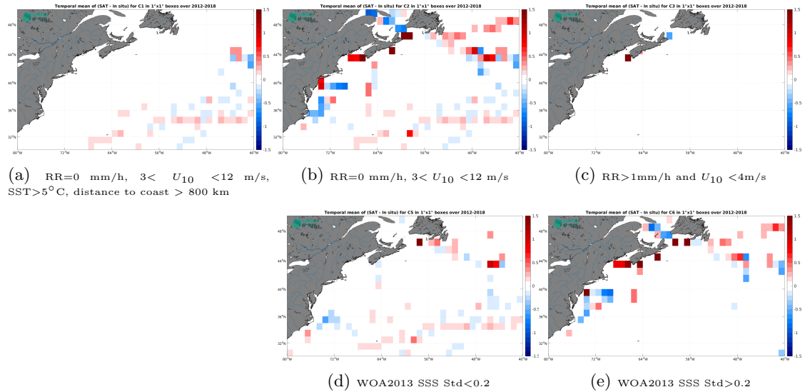
Figure 12: Temporal mean gridded over spatial boxes of size 1^{\circ}\times 1^{\circ} of \Delta SSS (SMOS SSS L3 v8 - 18 Days (CATDS-CEC-LOCEAN) - TSG (GOSUD-Sailing-ship)) for 5 different subdatasets corresponding to:RR=0 mm/h, 3 < U_{10} < 12 m/s, SST > 5^{\circ}\text{C} , distance to coast > 800 km (a), RR=0 mm/h, 3 < U_{10} < 12 m/s (b), RR > 1 mm/h and U_{10} < 4 m/s (c), WOA2013 SSS Std < 0.2 (d), WOA2013 SSS Std > 0.2 (e).
