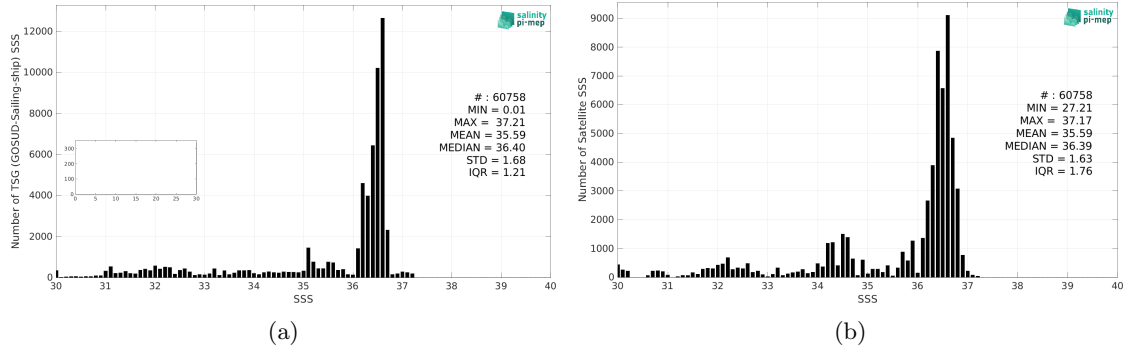
Figure 2: Histograms of SSS from TSG (GOSUD-Sailing-ship) (a) and SMOS SSS L3 v8 - 18 Days (CATDS-CEC-LOCEAN) (b) considering all match-up pairs per bins of 0.1 over the Gulf Stream Pi-MEP region and for the full satellite product period.
