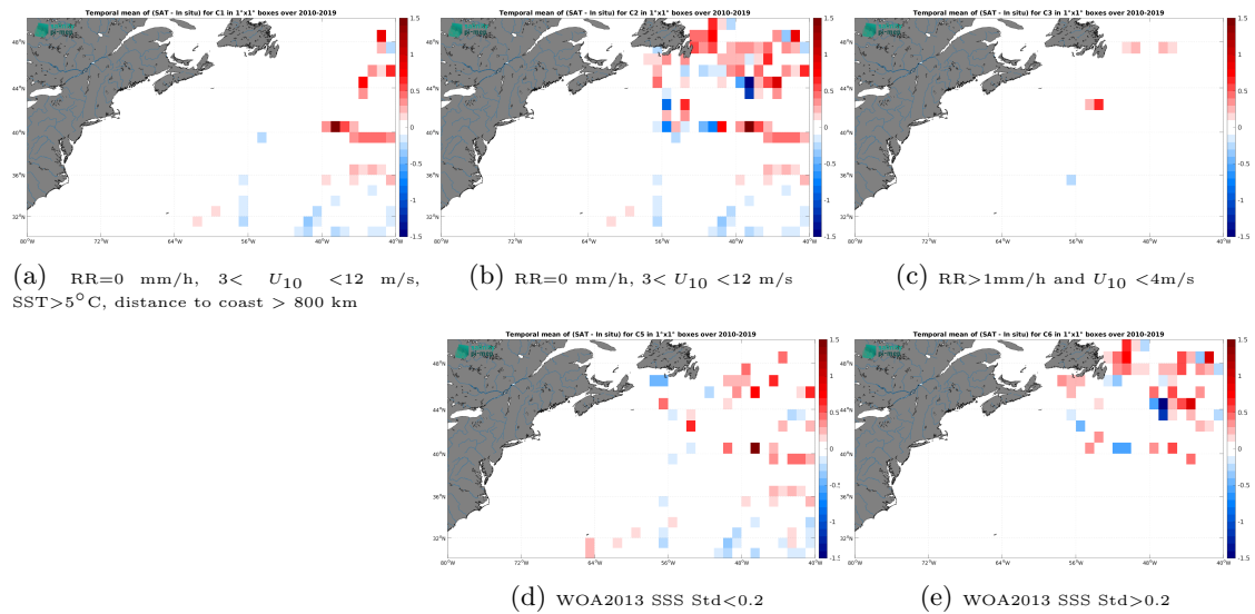
Figure 12: Temporal mean gridded over spatial boxes of size 1^{\circ}\times 1^{\circ} of \Delta SSS (SMOS SSS L3 v8 - 18 Days (CATDS-CEC-LOCEAN) - TSG (GOSUD-Research-vessel)) for 5 different subdatasets corresponding to:RR=0 mm/h, 3 < U_{10} < 12 m/s, SST > 5^{\circ}\text{C} , distance to coast > 800 km (a), RR=0 mm/h, 3 < U_{10} < 12 m/s (b), RR > 1 mm/h and U_{10} < 4 m/s (c), WOA2013 SSS Std < 0.2 (d), WOA2013 SSS Std > 0.2 (e).
