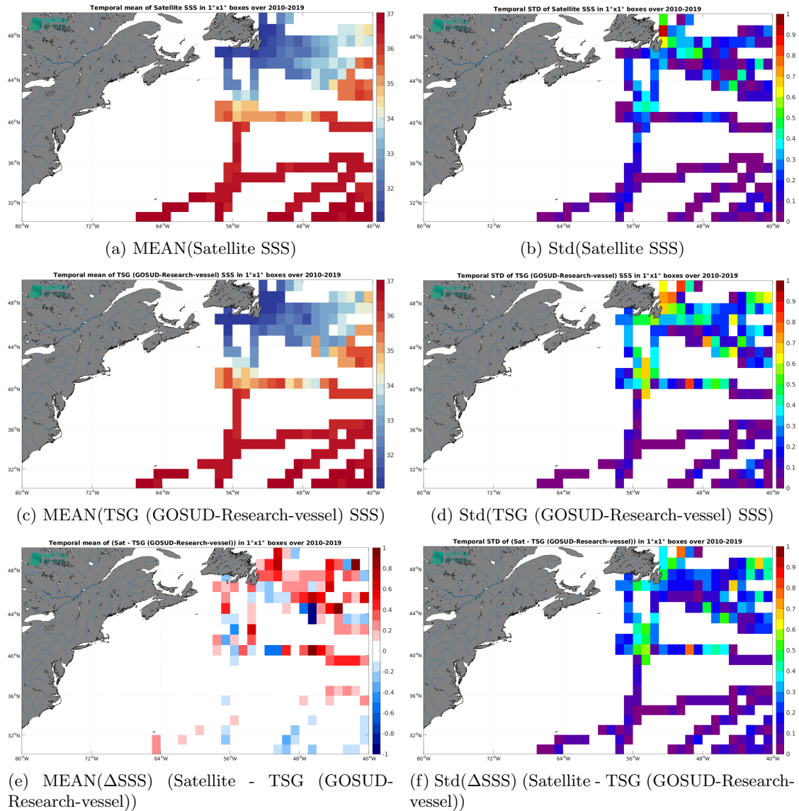
Figure 6: Temporal mean (left) and Std (right) of SSS from SMOS SSS L3 v8 - 18 Days (CATDS-CEC-LOCEAN) (top), TSG (GOSUD-Research-vessel) (middle), and of \Delta SSS (Satellite - TSG (GOSUD-Research-vessel)). Only match-up pairs are used to generate these maps.
