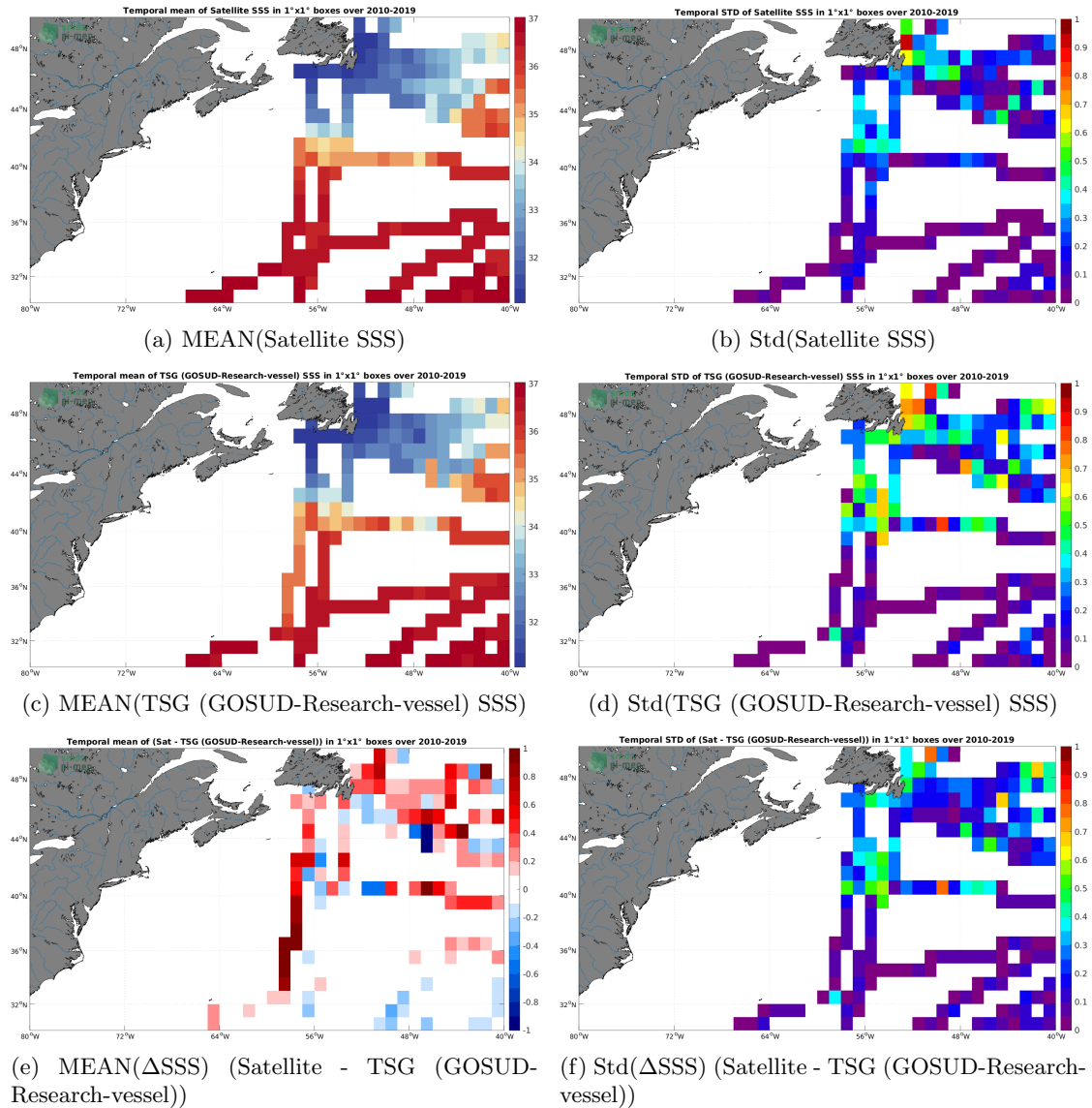
Figure 6: Temporal mean (left) and Std (right) of SSS from SMOS SSS L3 v8 - 18 Days (CATDS-CECOS-LOCEAN) (top), TSG (GOSUD-Research-vessel) (middle), and of \Delta SSS (Satellite - TSG (GOSUD-Research-vessel)). Only match-up pairs are used to generate these maps.
