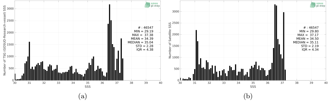
Figure 2: Histograms of SSS from TSG (GOSUD-Research-vessel) (a) and SMOS SSS L3 v8 - 18 Days (CATDS-CECOS-LOCEAN) (b) considering all match-up pairs per bins of 0.1 over the Gulf Stream Pi-MEP region and for the full satellite product period.
