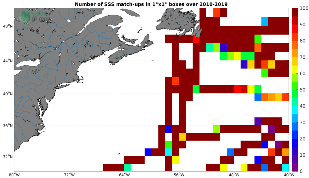
Figure 4: Number of SSS match-ups between TSG (GOSUD-Research-vessel) SSS and the SMOS SSS L3 v8 - 18 Days (CATDS-CECOS-LOCEAN) SSS product for the Gulf Stream Pi-MEP region over 1^\circ \times 1^\circ boxes and for the full satellite product period.
