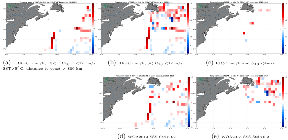
Figure 12: Temporal mean gridded over spatial boxes of size 1^{\circ}\times 1^{\circ} of \Delta SSS (SMOS SSS L3 v8 - 18 Days (CATDS-CECOS-LOCEAN) - TSG (GOSUD-Research-vessel)) for 5 different sub-datasets corresponding to:RR=0 mm/h, 3 < U_{10} < 12 m/s, SST > 5^{\circ}\text{C} , distance to coast > 800 km (a), RR=0 mm/h, 3 < U_{10} < 12 m/s (b), RR > 1 mm/h and U_{10} < 4 m/s (c), WOA2013 SSS Std < 0.2 (d), WOA2013 SSS Std > 0.2 (e).
