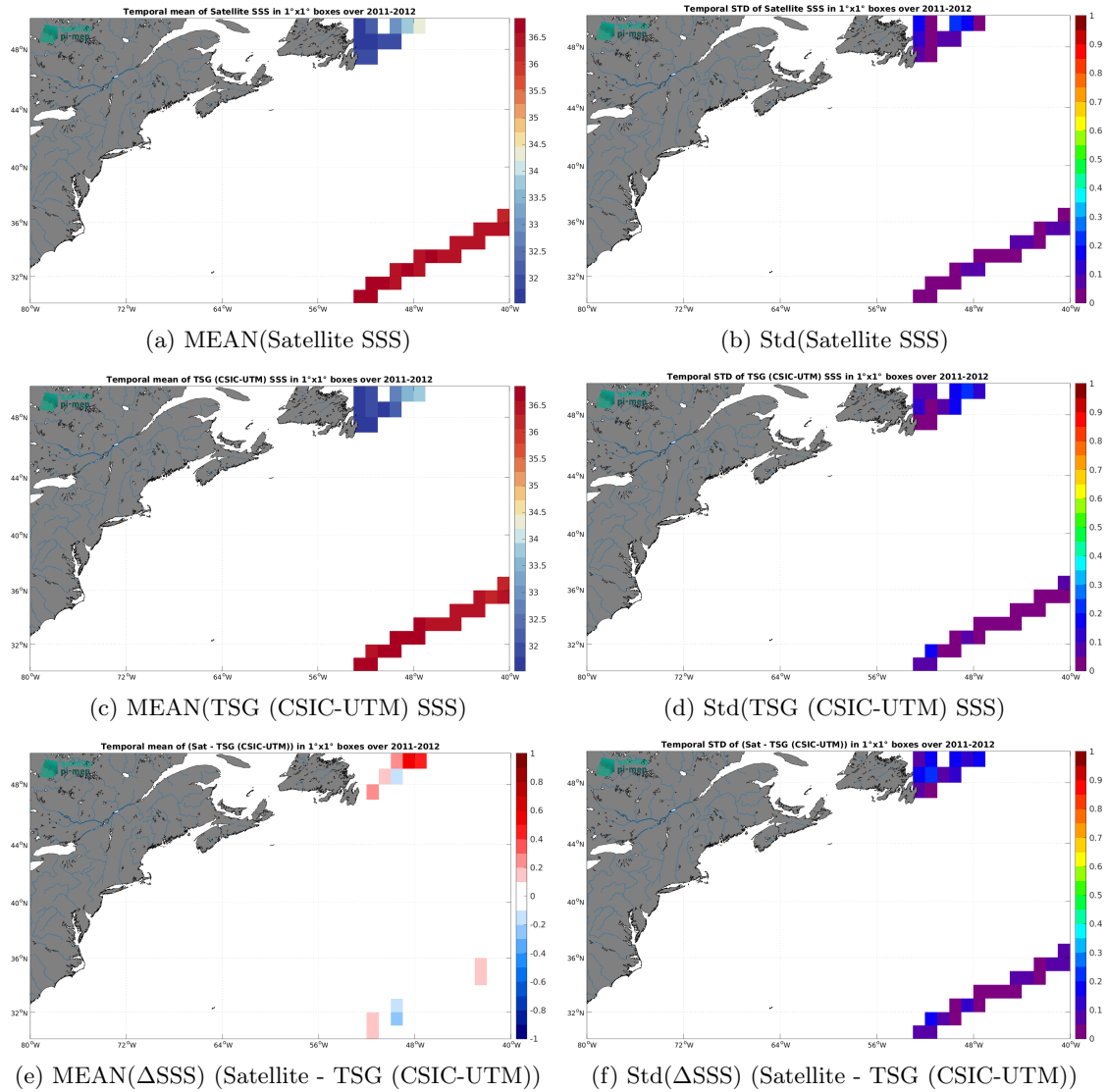
Figure 6: Temporal mean (left) and Std (right) of SSS from SMOS SSS L3 v8 - 18 Days (CATDS-CEC-LOCEAN) (top), TSG (CSIC-UTM) (middle), and of \Delta SSS (Satellite - TSG (CSIC-UTM)). Only match-up pairs are used to generate these maps.
