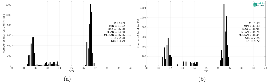
Figure 2: Histograms of SSS from TSG (CSIC-UTM) (a) and SMOS SSS L3 v8 - 18 Days (CATDS-CEC-LOCEAN) (b) considering all match-up pairs per bins of 0.1 over the Gulf Stream Pi-MEP region and for the full satellite product period.
