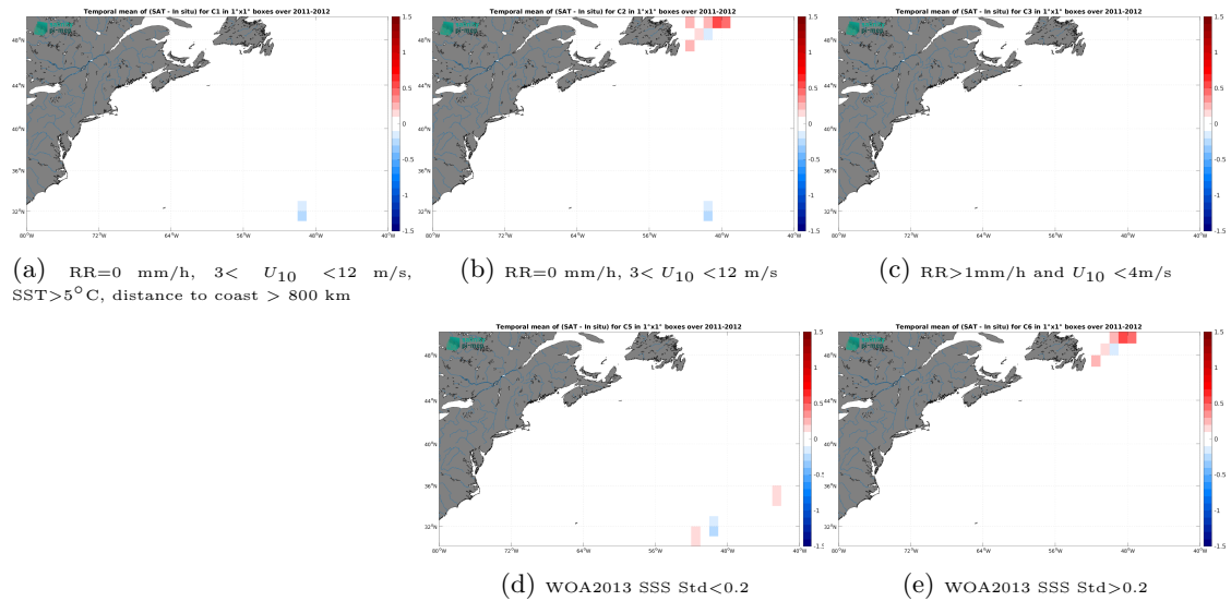
Figure 12: Temporal mean gridded over spatial boxes of size 1^{\circ}\times 1^{\circ} of \Delta\text{SSS} (SMOS SSS L3 v8 - 18 Days (CATDS-CEC-LOCEAN) - TSG (CSIC-UTM)) for 5 different subdatasets corresponding to:RR=0 mm/h, 3 < U_{10} < 12 m/s, SST >5^{\circ}\text{C} , distance to coast > 800 km (a), RR=0 mm/h, 3 < U_{10} < 12 m/s (b), RR >1 mm/h and U_{10} < 4 m/s (c), WOA2013 SSS Std <0.2 (d), WOA2013 SSS Std >0.2 (e).
