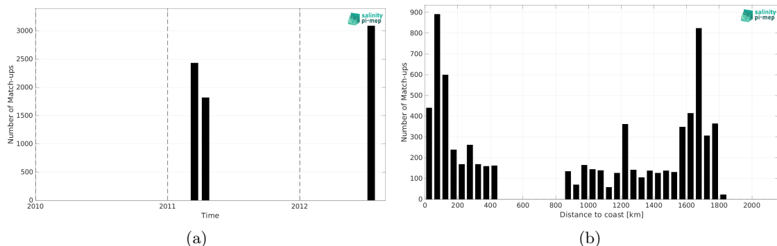
Figure 1: Number of match-ups between TSG (CSIC-UTM) and SMOS SSS L3 v8 - 18 Days (CATDS-CEC-LOCEAN) SSS as a function of time (a) and as function of the distance to coast (b) over the Gulf Stream Pi-MEP region and for the full satellite product period.
