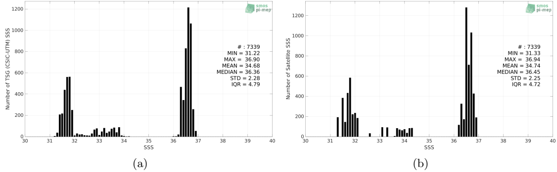
Figure 2: Histograms of SSS from TSG (CSIC-UTM) (a) and SMOS SSS L3 v8 - 18 Days (CATDS-CECOS-LOCEAN) (b) considering all match-up pairs per bins of 0.1 over the Gulf Stream Pi-MEP region and for the full satellite product period.
