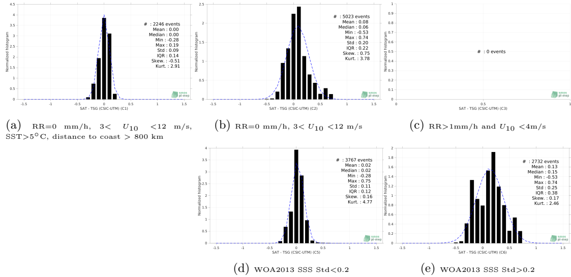
Figure 13: Normalized histogram of \Delta SSS (SMOS SSS L3 v8 - 18 Days (CATDS-CECOS-LOCEAN) - TSG (CSIC-UTM)) for 5 different subdatasets corresponding to: RR=0 mm/h, 3 < U_{10} < 12 m/s, SST > 5°C, distance to coast > 800 km (a), RR=0 mm/h, 3 < U_{10} < 12 m/s (b), RR > 1mm/h and U_{10} < 4 m/s (c), WOA2013 SSS Std < 0.2 (d), WOA2013 SSS Std > 0.2 (e).
