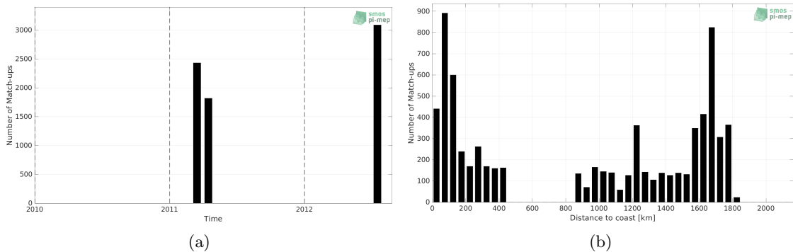
Figure 1: Number of match-ups between TSG (CSIC-UTM) and SMOS SSS L3 v8 - 18 Days (CATDS-CECOS-LOCEAN) SSS as a function of time (a) and as function of the distance to coast (b) over the Gulf Stream Pi-MEP region and for the full satellite product period.
