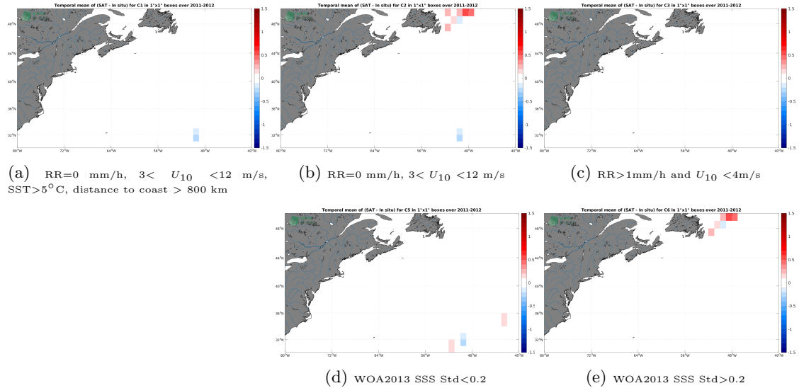
Figure 12: Temporal mean gridded over spatial boxes of size 1^{\circ}\times 1^{\circ} of \Delta\text{SSS} (SMOS SSS L3 v8 - 18 Days (CATDS-CECOS-LOCEAN) - TSG (CSIC-UTM)) for 5 different subdatasets corresponding to:RR=0 mm/h, 3 < U_{10} < 12 m/s, SST >5^{\circ}\text{C} , distance to coast > 800 km (a), RR=0 mm/h, 3 < U_{10} < 12 m/s (b), RR >1 mm/h and U_{10} < 4 m/s (c), WOA2013 SSS Std <0.2 (d), WOA2013 SSS Std >0.2 (e).
