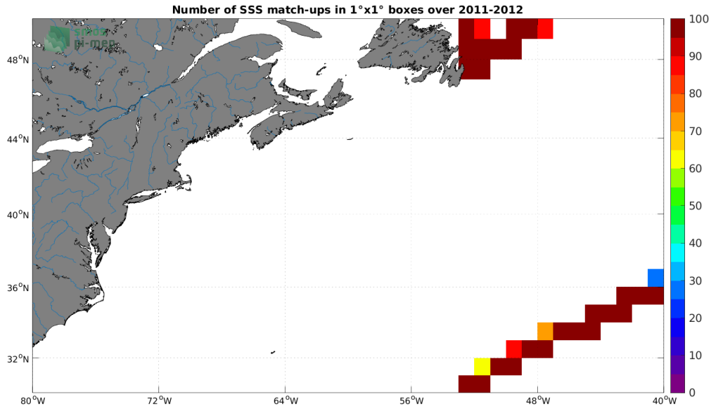
Figure 4: Number of SSS match-ups between TSG (CSIC-UTM) SSS and the SMOS SSS L3 v8 - 18 Days (CATDS-CECOS-LOCEAN) SSS product for the Gulf Stream Pi-MEP region over 1^\circ \times 1^\circ boxes and for the full satellite product period.
