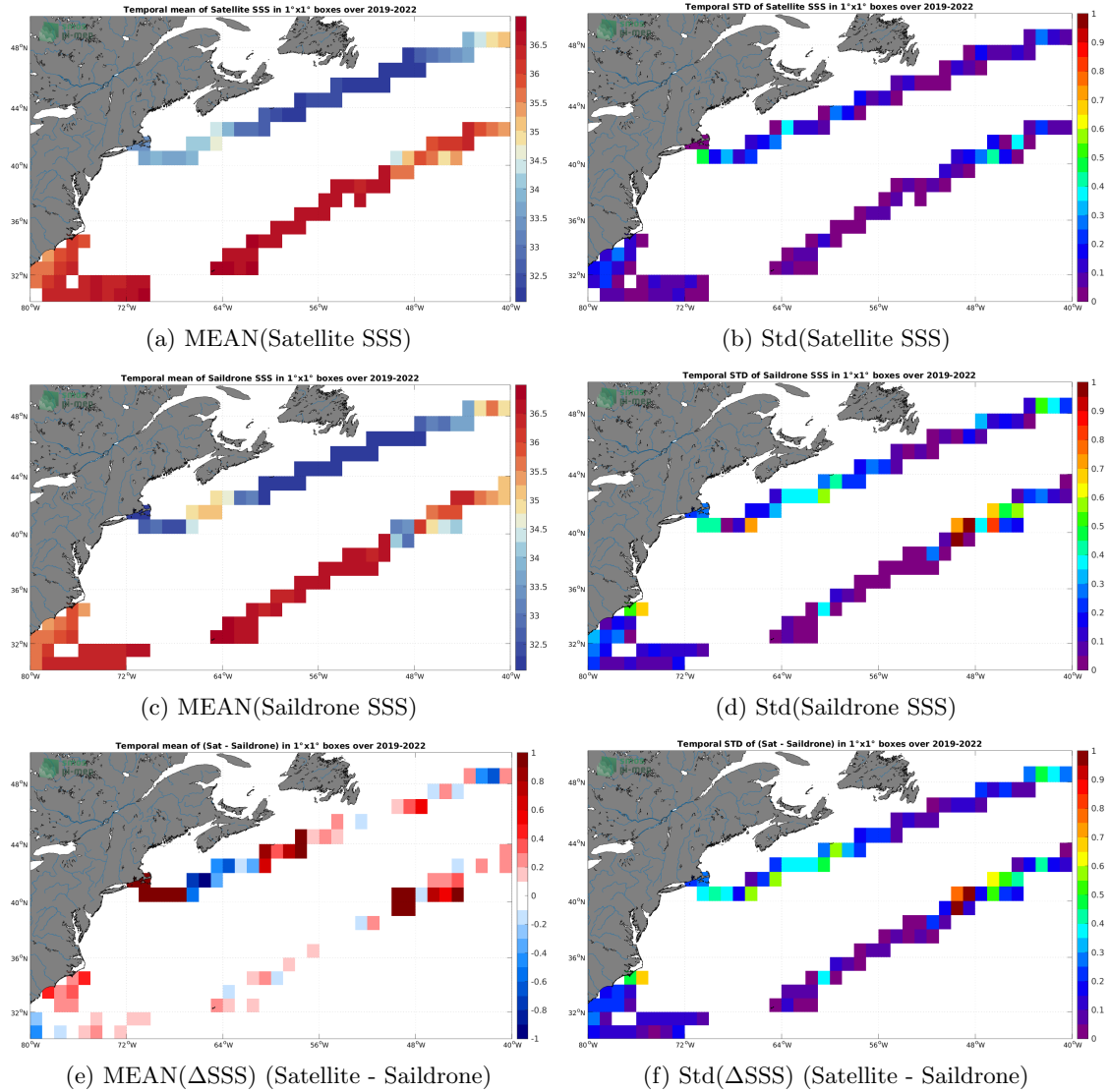
Figure 6: Temporal mean (left) and Std (right) of SSS from SMOS SSS L3 v8 - 18 Days (CATDS-CECOS-LOCEAN) (top), Saildrone (middle), and of \Delta SSS (Satellite - Saildrone). Only match-up pairs are used to generate these maps.
