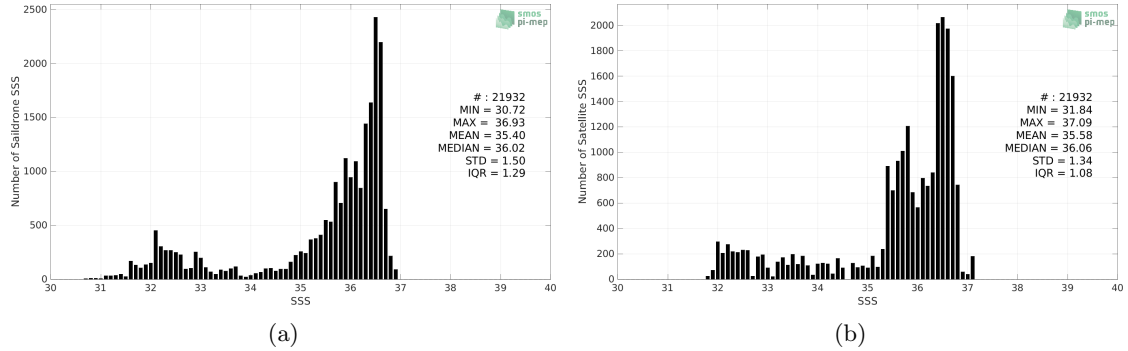
Figure 2: Histograms of SSS from Saildrone (a) and SMOS SSS L3 v8 - 18 Days (CATDS-CECOS-LOCEAN) (b) considering all match-up pairs per bins of 0.1 over the Gulf Stream Pi-MEP region and for the full satellite product period.
