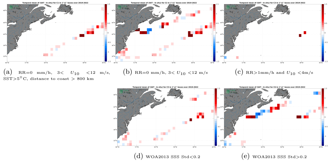
Figure 12: Temporal mean gridded over spatial boxes of size 1^\circ \times 1^\circ of \Delta SSS (SMOS SSS L3 v8 - 18 Days (CATDS-CECOS-LOCEAN) - Sairdrone) for 5 different subdatasets corresponding to:RR=0 mm/h, 3 < U_{10} < 12 m/s, SST >5^\circ C, distance to coast > 800 km (a), RR=0 mm/h, 3 < U_{10} < 12 m/s (b), RR >1 mm/h and U_{10} < 4 m/s (c), WOA2013 SSS Std <0.2 (d), WOA2013 SSS Std >0.2 (e).
