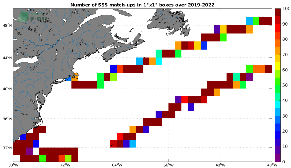
Figure 4: Number of SSS match-ups between Saildrone SSS and the SMOS SSS L3 v8 - 18 Days (CATDS-CECOS-LOCEAN) SSS product for the Gulf Stream Pi-MEP region over 1^\circ \times 1^\circ boxes and for the full satellite product period.
