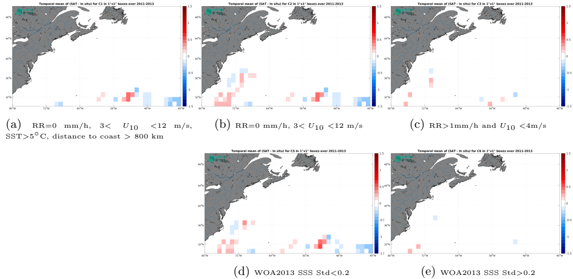
Figure 11: Temporal mean gridded over spatial boxes of size 1^{\circ}\times 1^{\circ} of \Delta\text{SSS} (SMOS SSS L3 v8 - 18 Days (CATDS-CEC-LOCEAN) - Surface drifters) for 5 different subdatasets corresponding to:RR=0 mm/h, 3 < U_{10} < 12 m/s, SST >5^{\circ}\text{C} , distance to coast > 800 km (a), RR=0 mm/h, 3 < U_{10} < 12 m/s (b), RR >1 mm/h and U_{10} < 4 m/s (c), WOA2013 SSS Std <0.2 (d), WOA2013 SSS Std >0.2 (e).
