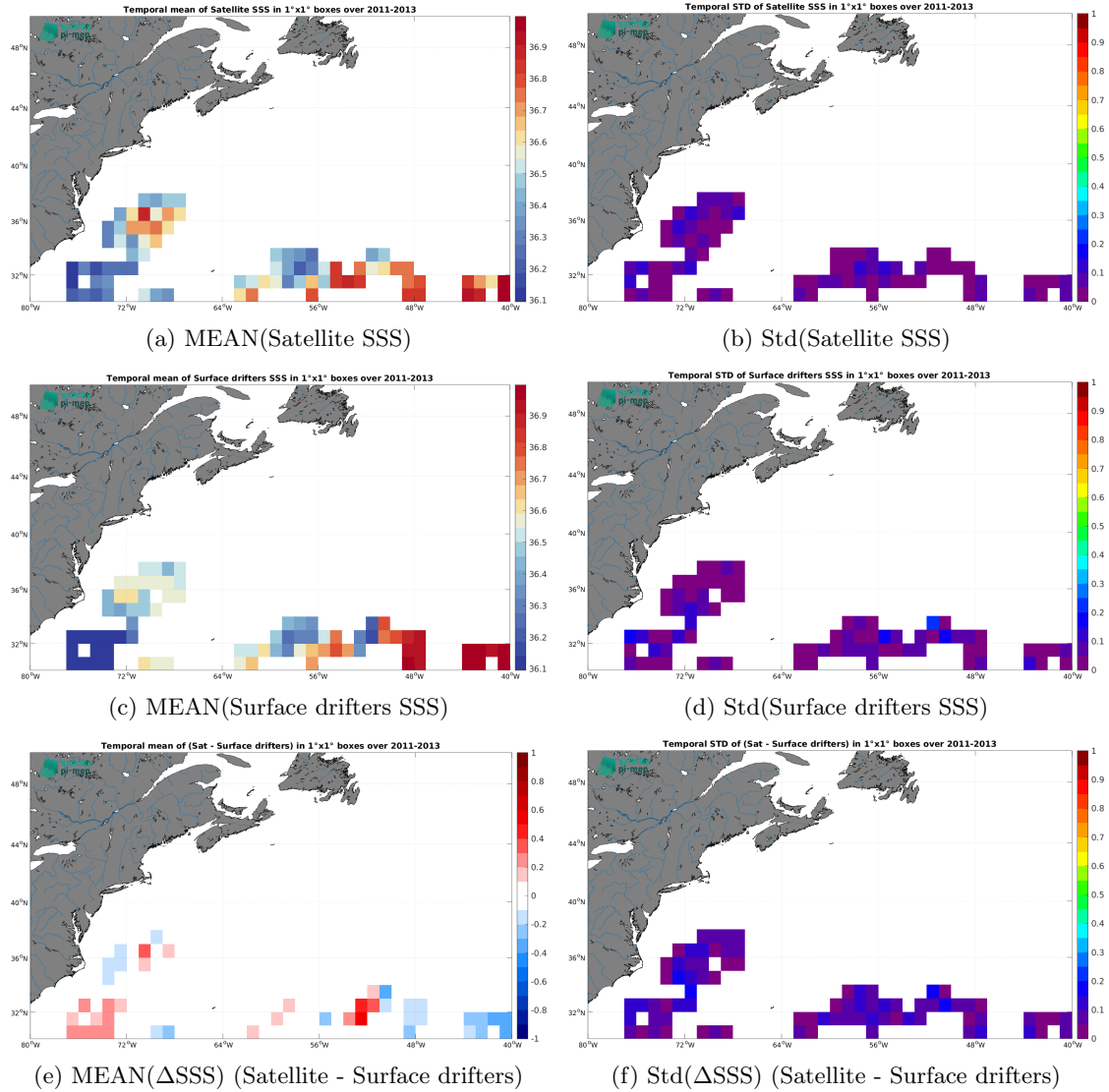
Figure 5: Temporal mean (left) and Std (right) of SSS from SMOS SSS L3 v8 - 18 Days (CATDS-CEC-LOCEAN) (top), Surface drifters (middle), and of \Delta SSS (Satellite - Surface drifters). Only match-up pairs are used to generate these maps.
