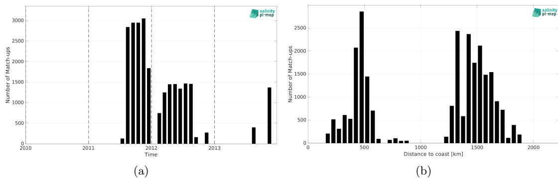
Figure 1: Number of match-ups between Surface drifters and SMOS SSS L3 v8 - 18 Days (CATDS-CEC-LOCEAN) SSS as a function of time (a) and as function of the distance to coast (b) over the Gulf Stream Pi-MEP region and for the full satellite product period.
