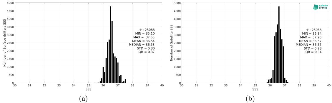
Figure 2: Histograms of SSS from Surface drifters (a) and SMOS SSS L3 v8 - 18 Days (CATDS-CEC-LOCEAN) (b) considering all match-up pairs per bins of 0.1 over the Gulf Stream Pi-MEP region and for the full satellite product period.
