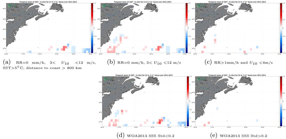
Figure 11: Temporal mean gridded over spatial boxes of size 1^{\circ}\times 1^{\circ} of \Delta\text{SSS} (SMOS SSS L3 v8 - 18 Days (CATDS-CECOS-LOCEAN) - Surface drifters) for 5 different subdatasets corresponding to:RR=0 mm/h, 3 < U_{10} < 12 m/s, SST >5^{\circ}\text{C} , distance to coast > 800 km (a), RR=0 mm/h, 3 < U_{10} < 12 m/s (b), RR >1 mm/h and U_{10} < 4 m/s (c), WOA2013 SSS Std <0.2 (d), WOA2013 SSS Std >0.2 (e).
