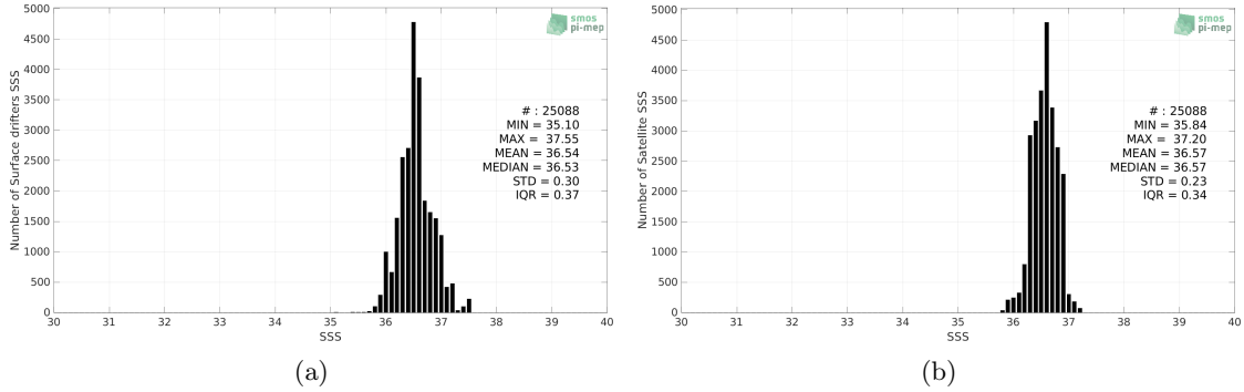
Figure 2: Histograms of SSS from Surface drifters (a) and SMOS SSS L3 v8 - 18 Days (CATDS-CECOS-LOCEAN) (b) considering all match-up pairs per bins of 0.1 over the Gulf Stream Pi-MEP region and for the full satellite product period.
