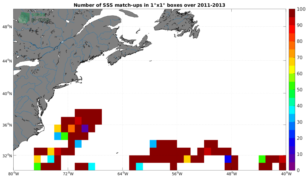
Figure 3: Number of SSS match-ups between Surface drifters SSS and the SMOS SSS L3 v8 - 18 Days (CATDS-CECOS-LOCEAN) SSS product for the Gulf Stream Pi-MEP region over 1^\circ \times 1^\circ boxes and for the full satellite product period.
