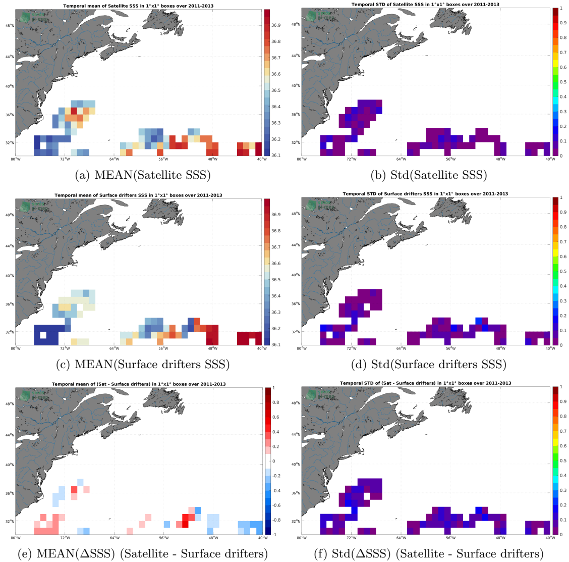
Figure 5: Temporal mean (left) and Std (right) of SSS from SMOS SSS L3 v8 - 18 Days (CATDS-CECOS-LOCEAN) (top), Surface drifters (middle), and of \Delta SSS (Satellite - Surface drifters). Only match-up pairs are used to generate these maps.
