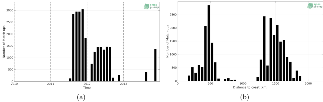
Figure 1: Number of match-ups between Surface drifters and SMOS SSS L3 v8 - 18 Days (CATDS-CECOS-LOCEAN) SSS as a function of time (a) and as function of the distance to coast (b) over the Gulf Stream Pi-MEP region and for the full satellite product period.
