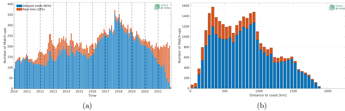
Figure 1: Number of match-ups between Argo and SMOS SSS L3 v7 - 9 Days (CATDS-CECOS-LOCEAN) SSS as a function of time (a) and as function of the distance to coast (b) over the Gulf Stream Pi-MEP region and for the full satellite product period.
