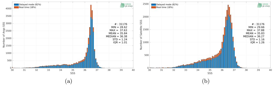
Figure 2: Histograms of SSS from Argo (a) and SMOS SSS L3 v7 - 9 Days (CATDS-CECOS-LOCEAN) (b) considering all match-up pairs per bins of 0.1 over the Gulf Stream Pi-MEP region and for the full satellite product period.
