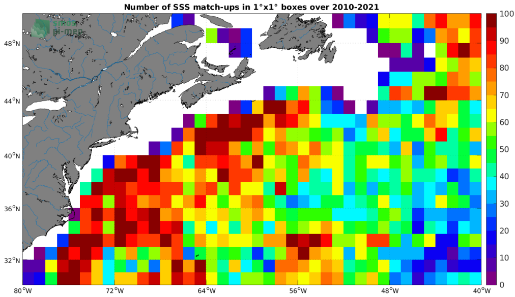
Figure 4: Number of SSS match-ups between Argo SSS and the SMOS SSS L3 v7 - 9 Days (CATDS-CECOS-LOCEAN) SSS product for the Gulf Stream Pi-MEP region over 1^\circ \times 1^\circ boxes and for the full satellite product period.
