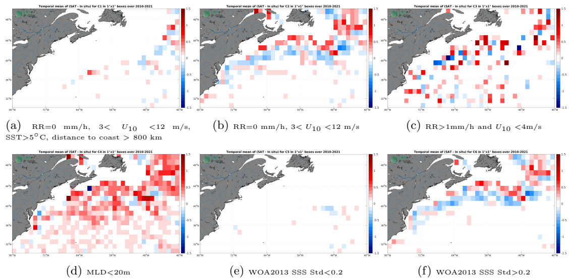
Figure 12: Temporal mean gridded over spatial boxes of size 1^\circ \times 1^\circ of \Delta SSS (SMOS SSS L3 v7 - 9 Days (CATDS-CECOS-LOCEAN) - Argo) for 6 different subdatasets corresponding to:RR=0 mm/h, 3 < U_{10} < 12 m/s, SST > 5^\circ\text{C} , distance to coast > 800 km (a), RR=0 mm/h, 3 < U_{10} < 12 m/s (b), RR > 1 mm/h and U_{10} < 4 m/s (c),MLD < 20 m (d),WOA2013 SSS Std < 0.2 (e),WOA2013 SSS Std > 0.2 (f).
