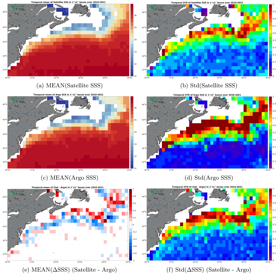
Figure 6: Temporal mean (left) and Std (right) of SSS from SMOS SSS L3 v7 - 9 Days (CATDS-CECOS-LOCEAN) (top), Argo (middle), and of \Delta SSS (Satellite - Argo). Only match-up pairs are used to generate these maps.
