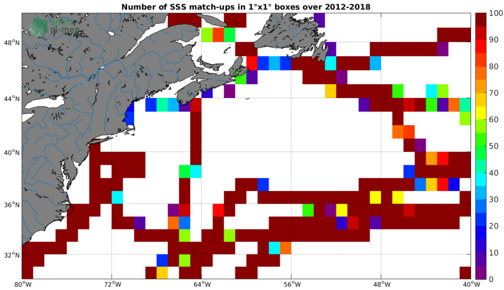
Figure 4: Number of SSS match-ups between TSG (GOSUD-Sailing-ship) SSS and the SMOS SSS L3 v5 - 9 Days (CATDS-CECOS-LOCEAN) SSS product for the Gulf Stream Pi-MEP region over 1^{\circ} \times 1^{\circ} boxes and for the full satellite product period.
