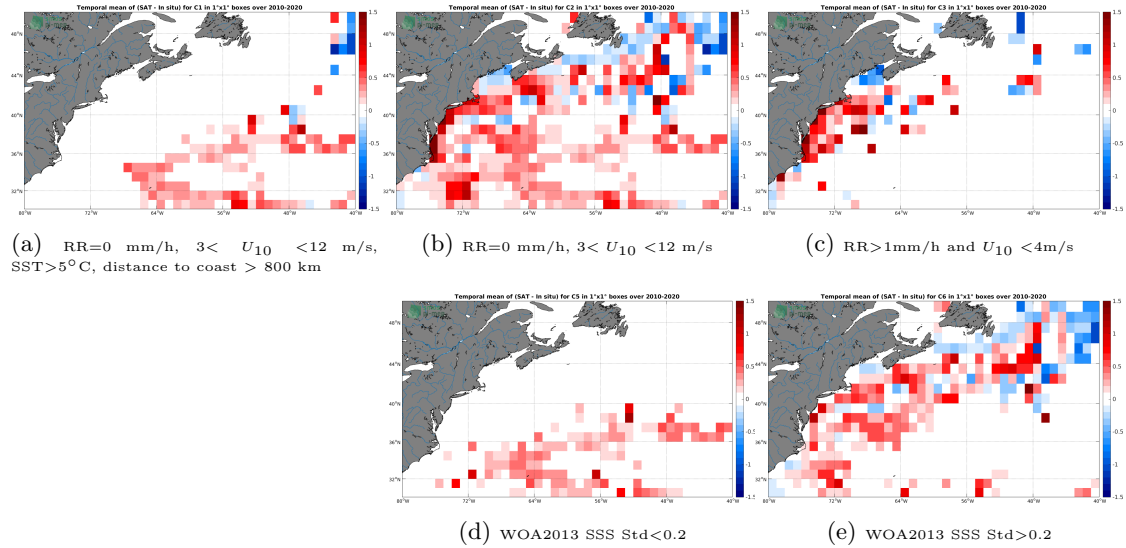
Figure 12: Temporal mean gridded over spatial boxes of size 1^{\circ}\times 1^{\circ} of \Delta\text{SSS} (SMOS SSS L3 v5 - 18 Days (CATDS-CECOS-LOCEAN) - TSG (SAMOS)) for 5 different subdatasets corresponding to:RR=0 mm/h, 3 < U_{10} < 12 m/s, SST >5^{\circ}\text{C} , distance to coast > 800 km (a), RR=0 mm/h, 3 < U_{10} < 12 m/s (b), RR >1 mm/h and U_{10} < 4 m/s (c), WOA2013 SSS Std <0.2 (d), WOA2013 SSS Std >0.2 (e).
