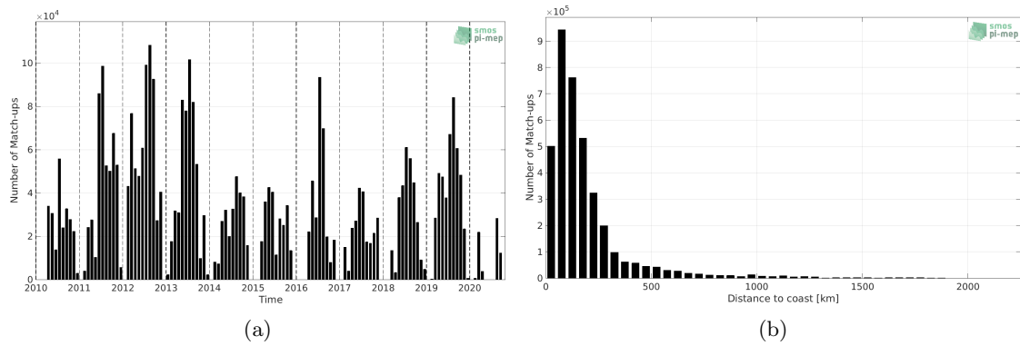
Figure 1: Number of match-ups between TSG (SAMOS) and SMOS SSS L3 v5 - 18 Days (CATDS-CECOS-LOCEAN) SSS as a function of time (a) and as function of the distance to coast (b) over the Gulf Stream Pi-MEP region and for the full satellite product period.
