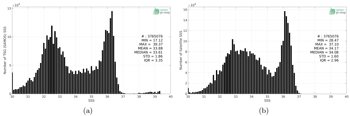
Figure 2: Histograms of SSS from TSG (SAMOS) (a) and SMOS SSS L3 v5 - 18 Days (CATDS-CECOS-LOCEAN) (b) considering all match-up pairs per bins of 0.1 over the Gulf Stream Pi-MEP region and for the full satellite product period.
