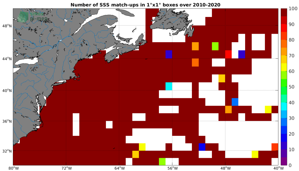
Figure 4: Number of SSS match-ups between TSG (SAMOS) SSS and the SMOS SSS L3 v5 - 18 Days (CATDS-CECOS-LOCEAN) SSS product for the Gulf Stream Pi-MEP region over 1^\circ \times 1^\circ boxes and for the full satellite product period.
