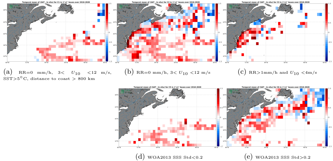
Figure 12: Temporal mean gridded over spatial boxes of size 1^{\circ}\times 1^{\circ} of \Delta\text{SSS} (SMOS SSS L3 v5 - 18 Days (CATDS-CECOS-LOCEAN) - TSG (SAMOS)) for 5 different subdatasets corresponding to:RR=0 mm/h, 3 < U_{10} < 12 m/s, SST >5^{\circ}\text{C} , distance to coast > 800 km (a), RR=0 mm/h, 3 < U_{10} < 12 m/s (b), RR >1 mm/h and U_{10} < 4 m/s (c), WOA2013 SSS Std <0.2 (d), WOA2013 SSS Std >0.2 (e).
