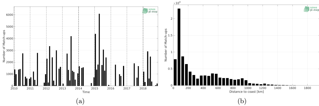
Figure 1: Number of match-ups between TSG (LEGOS-DM) and SMOS SSS L3 v5 - 18 Days (CATDS-CECOS-LOCEAN) SSS as a function of time (a) and as function of the distance to coast (b) over the Gulf Stream Pi-MEP region and for the full satellite product period.
