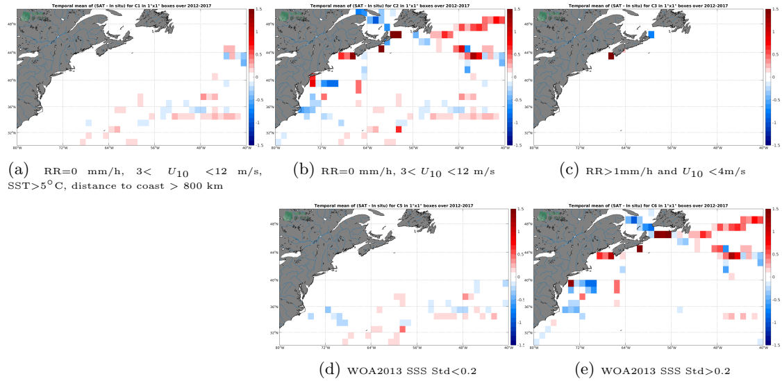
Figure 12: Temporal mean gridded over spatial boxes of size 1^{\circ}\times 1^{\circ} of \Delta SSS (SMOS SSS L3 v5 - 18 Days (CATDS-CECOS-LOCEAN) - TSG (GOSUD-Sailing-ship)) for 5 different subdatasets corresponding to:RR=0 mm/h, 3 < U_{10} < 12 m/s, SST > 5^{\circ}\text{C} , distance to coast > 800 km (a), RR=0 mm/h, 3 < U_{10} < 12 m/s (b), RR > 1 mm/h and U_{10} < 4 m/s (c), WOA2013 SSS Std < 0.2 (d), WOA2013 SSS Std > 0.2 (e).
