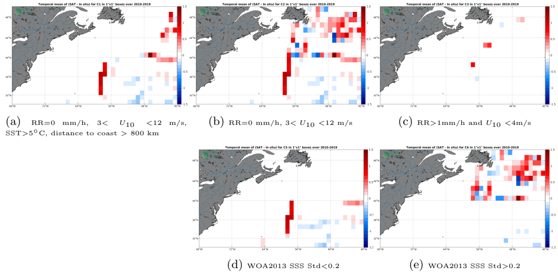
Figure 12: Temporal mean gridded over spatial boxes of size 1^\circ \times 1^\circ of \Delta SSS (SMOS SSS L3 v5 - 18 Days (CATDS-CECOS-LOCEAN) - TSG (GOSUD-Research-vessel)) for 5 different sub-datasets corresponding to: RR=0 mm/h, 3 < U_{10} < 12 m/s, SST > 5^\circ\text{C} , distance to coast > 800 km (a), RR=0 mm/h, 3 < U_{10} < 12 m/s (b), RR > 1 mm/h and U_{10} < 4 m/s (c), WOA2013 SSS Std < 0.2 (d), WOA2013 SSS Std > 0.2 (e).
