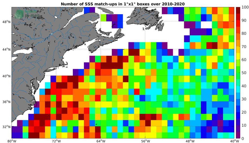
Figure 4: Number of SSS match-ups between Argo SSS and the SMOS SSS L3 v5 - 18 Days (CATDS-CECOS-LOCEAN) SSS product for the Gulf Stream Pi-MEP region over 1^\circ \times 1^\circ boxes and for the full satellite product period.
