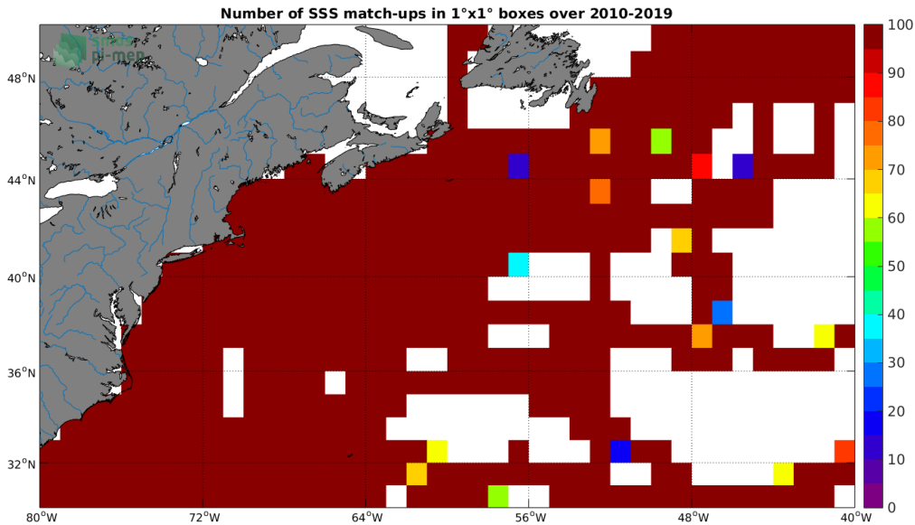
Figure 4: Number of SSS match-ups between TSG-SAMOS SSS and the SMOS-L3-CATDS-CECOS-LOCEAN-V4-9DAYS-25KM SSS product for the Gulf Stream Pi-MEP region over 1°x1° boxes and for the full satellite product period.
