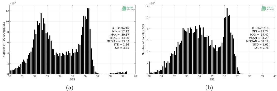
Figure 2: Histograms of SSS from TSG-SAMOS (a) and SMOS-L3-CATDS-CECOS-LOCEAN-V4-9DAYS-25KM (b) considering all match-up pairs per bins of 0.1 over the Gulf Stream Pi-MEP region and for the full satellite product period.
