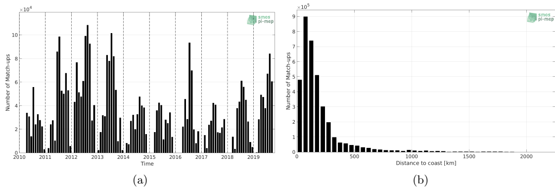
Figure 1: Number of match-ups between TSG-SAMOS and SMOS-L3-CATDS-CECOS-LOCEAN-V4-9DAYS-25KM SSS as a function of time (a) and as function of the distance to coast (b) over the Gulf Stream Pi-MEP region and for the full satellite product period.
