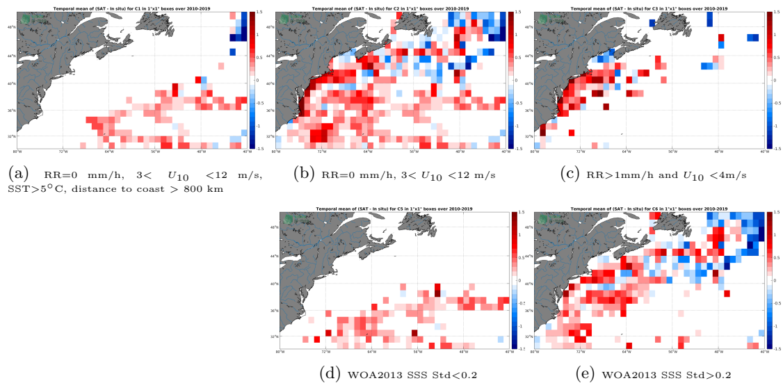
Figure 12: Temporal mean gridded over spatial boxes of size 1^{\circ}\times 1^{\circ} of \Delta\text{SSS} (SMOS-L3-CATDS-CECOS-LOCEAN-V4-9DAYS-25KM - TSG-SAMOS) for 5 different subdatasets corresponding to:RR=0 mm/h, 3 < U_{10} < 12 m/s, SST >5^{\circ}\text{C} , distance to coast > 800 km (a), RR=0 mm/h, 3 < U_{10} < 12 m/s (b), RR >1 mm/h and U_{10} < 4 m/s (c), WOA2013 SSS Std <0.2 (d), WOA2013 SSS Std >0.2 (e).
