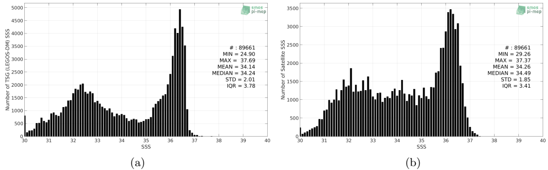
Figure 2: Histograms of SSS from TSG (LEGOS-DM) (a) and SMOS SSS L3 v4 - 9 Days (CATDS-CECOS-LOCEAN) (b) considering all match-up pairs per bins of 0.1 over the Gulf Stream Pi-MEP region and for the full satellite product period.
