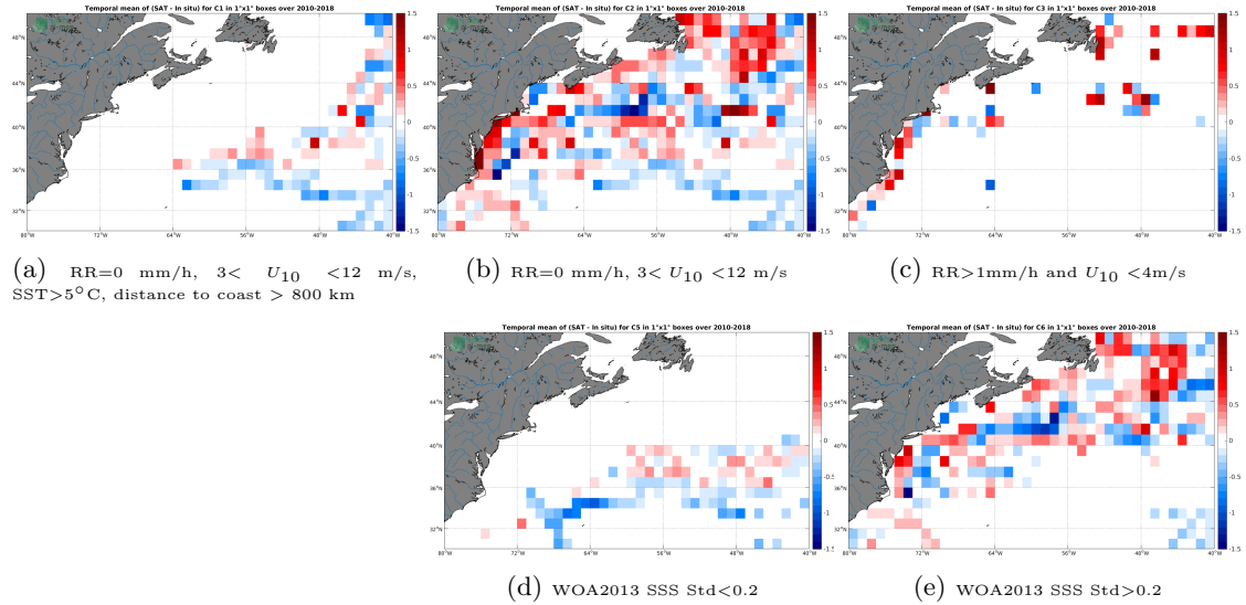
Figure 12: Temporal mean gridded over spatial boxes of size 1^{\circ}\times 1^{\circ} of \Delta\text{SSS} (SMOS SSS L3 v4 - 9 Days (CATDS-CECOS-LOCEAN) - TSG (LEGOS-DM)) for 5 different subdatasets corresponding to:RR=0 mm/h, 3 < U_{10} < 12 m/s, SST >5^{\circ}\text{C} , distance to coast > 800 km (a), RR=0 mm/h, 3 < U_{10} < 12 m/s (b), RR >1 mm/h and U_{10} < 4 m/s (c), WOA2013 SSS Std <0.2 (d), WOA2013 SSS Std >0.2 (e).
