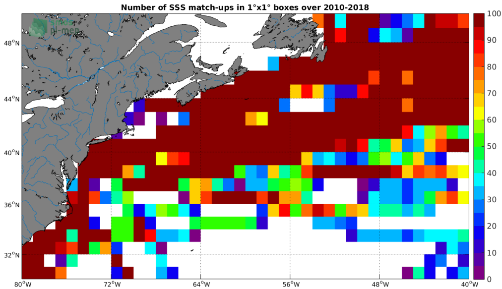
Figure 4: Number of SSS match-ups between TSG (LEGOS-DM) SSS and the SMOS SSS L3 v4 - 9 Days (CATDS-CECOS-LOCEAN) SSS product for the Gulf Stream Pi-MEP region over 1^\circ \times 1^\circ boxes and for the full satellite product period.
