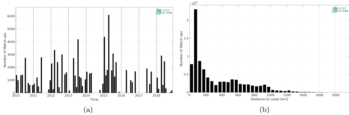
Figure 1: Number of match-ups between TSG (LEGOS-DM) and SMOS SSS L3 v4 - 9 Days (CATDS-CECOS-LOCEAN) SSS as a function of time (a) and as function of the distance to coast (b) over the Gulf Stream Pi-MEP region and for the full satellite product period.
