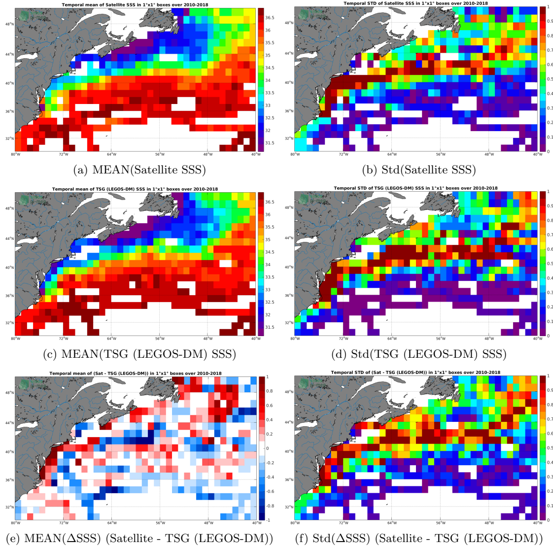
Figure 6: Temporal mean (left) and Std (right) of SSS from SMOS SSS L3 v4 - 9 Days (CATDS-CECOS-LOCEAN) (top), TSG (LEGOS-DM) (middle), and of \Delta SSS (Satellite - TSG (LEGOS-DM)). Only match-up pairs are used to generate these maps.
