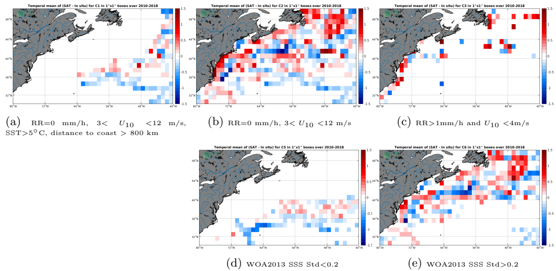
Figure 12: Temporal mean gridded over spatial boxes of size 1^\circ \times 1^\circ of \Delta SSS (SMOS-L3-CATDS-CECOS-LOCEAN-V4-9DAYS-25KM - TSG-LEGOS-DM) for 5 different subdatasets corresponding to:RR=0 mm/h, 3 < U_{10} < 12 m/s, SST >5^\circ\text{C} , distance to coast > 800 km (a), RR=0 mm/h, 3 < U_{10} < 12 m/s (b), RR >1 mm/h and U_{10} < 4 m/s (c), WOA2013 SSS Std <0.2 (d), WOA2013 SSS Std >0.2 (e).
