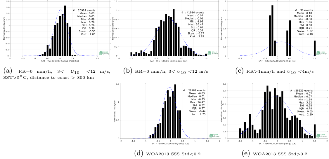
Figure 13: Normalized histogram of \Delta\text{SSS} (SMOS SSS L3 v4 - 9 Days (CATDS-CECOS-LOCEAN) - TSG (GOSUD-Sailing-ship)) for 5 different subdatasets corresponding to: RR=0 mm/h, 3 < U_{10} < 12 m/s, SST > 5^\circ\text{C} , distance to coast > 800 km (a), RR=0 mm/h, 3 < U_{10} < 12 m/s (b), RR > 1\text{mm/h} and U_{10} < 4\text{m/s} (c), WOA2013 SSS Std < 0.2 (d), WOA2013 SSS Std > 0.2 (e).
