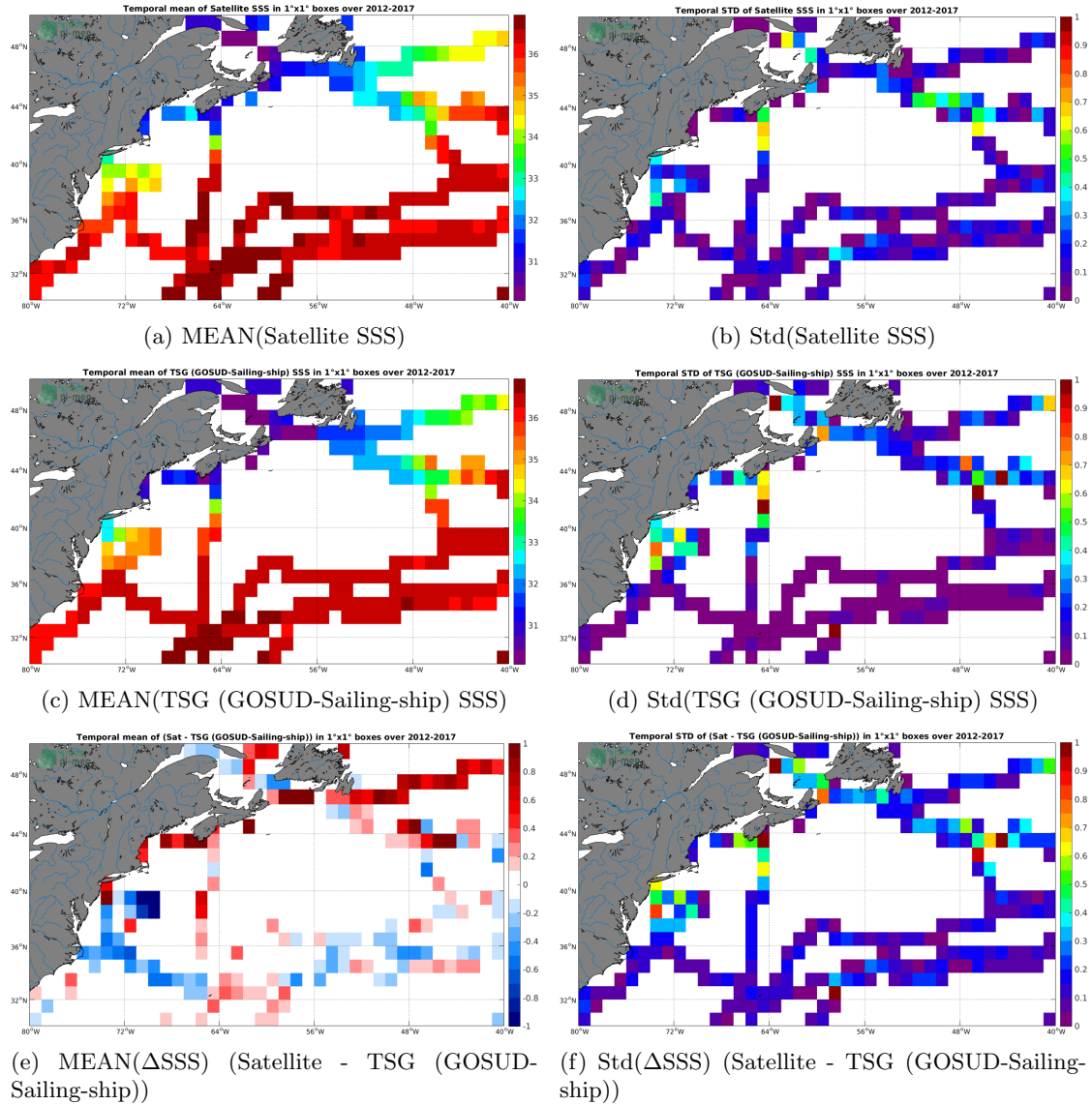
Figure 6: Temporal mean (left) and Std (right) of SSS from SMOS SSS L3 v4 - 9 Days (CATDS-CECOS-LOCEAN) (top), TSG (GOSUD-Sailing-ship) (middle), and of \Delta SSS (Satellite - TSG (GOSUD-Sailing-ship)). Only match-up pairs are used to generate these maps.
