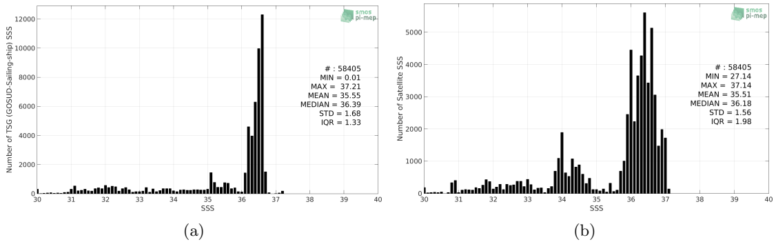
Figure 2: Histograms of SSS from TSG (GOSUD-Sailing-ship) (a) and SMOS SSS L3 v4 - 9 Days (CATDS-CECOS-LOCEAN) (b) considering all match-up pairs per bins of 0.1 over the Gulf Stream Pi-MEP region and for the full satellite product period.
