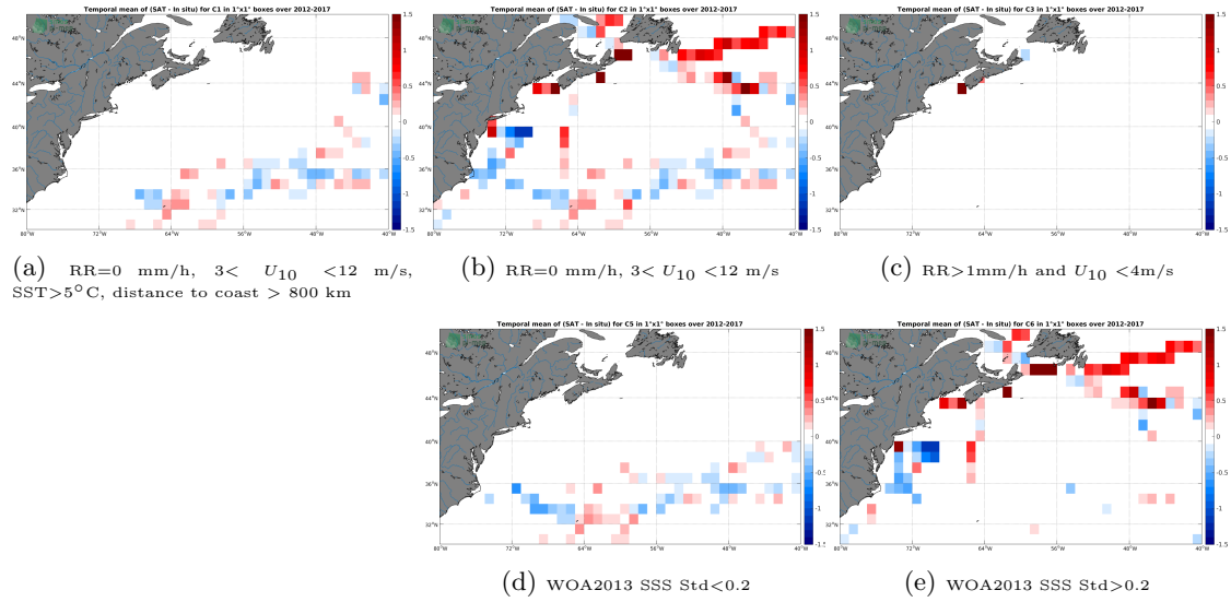
Figure 12: Temporal mean gridded over spatial boxes of size 1^\circ \times 1^\circ of \Delta SSS (SMOS SSS L3 v4 - 9 Days (CATDS-CECOS-LOCEAN) - TSG (GOSUD-Sailing-ship)) for 5 different subdatasets corresponding to:RR=0 mm/h, 3 < U_{10} < 12 m/s, SST >5^\circ\text{C} , distance to coast > 800 km (a), RR=0 mm/h, 3 < U_{10} < 12 m/s (b), RR >1 mm/h and U_{10} < 4 m/s (c), WOA2013 SSS Std <0.2 (d), WOA2013 SSS Std >0.2 (e).
