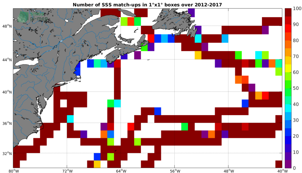
Figure 4: Number of SSS match-ups between TSG (GOSUD-Sailing-ship) SSS and the SMOS SSS L3 v4 - 9 Days (CATDS-CECOS-LOCEAN) SSS product for the Gulf Stream Pi-MEP region over 1^\circ \times 1^\circ boxes and for the full satellite product period.
