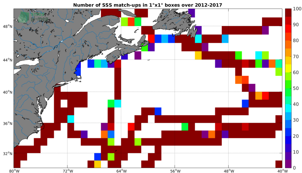
Figure 4: Number of SSS match-ups between TSG-GOSUD-Sailing-ship SSS and the SMOS-L3-CATDS-CECOS-LOCEAN-V4-9DAYS-25KM SSS product for the Gulf Stream Pi-MEP region over 1^\circ \times 1^\circ boxes and for the full satellite product period.
