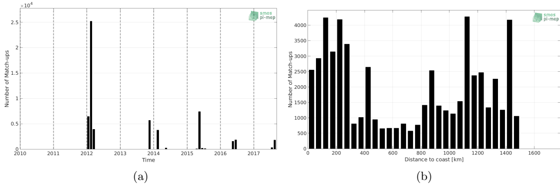
Figure 1: Number of match-ups between TSG-GOSUD-Sailing-ship and SMOS-L3-CATDS-CECOS-LOCEAN-V4-9DAYS-25KM SSS as a function of time (a) and as function of the distance to coast (b) over the Gulf Stream Pi-MEP region and for the full satellite product period.
