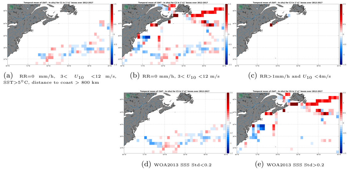
Figure 12: Temporal mean gridded over spatial boxes of size 1^\circ \times 1^\circ of \Delta SSS (SMOS-L3-CATDS-CECOS-LOCEAN-V4-9DAYS-25KM - TSG-GOSUD-Sailing-ship) for 5 different subdatasets corresponding to:RR=0 mm/h, 3 < U_{10} < 12 m/s, SST >5^\circ\text{C} , distance to coast > 800 km (a), RR=0 mm/h, 3 < U_{10} < 12 m/s (b), RR >1 mm/h and U_{10} < 4 m/s (c), WOA2013 SSS Std <0.2 (d), WOA2013 SSS Std >0.2 (e).
