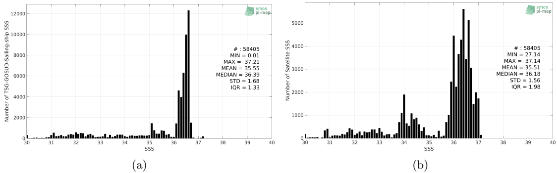
Figure 2: Histograms of SSS from TSG-GOSUD-Sailing-ship (a) and SMOS-L3-CATDS-CECOS-LOCEAN-V4-9DAYS-25KM (b) considering all match-up pairs per bins of 0.1 over the Gulf Stream Pi-MEP region and for the full satellite product period.
