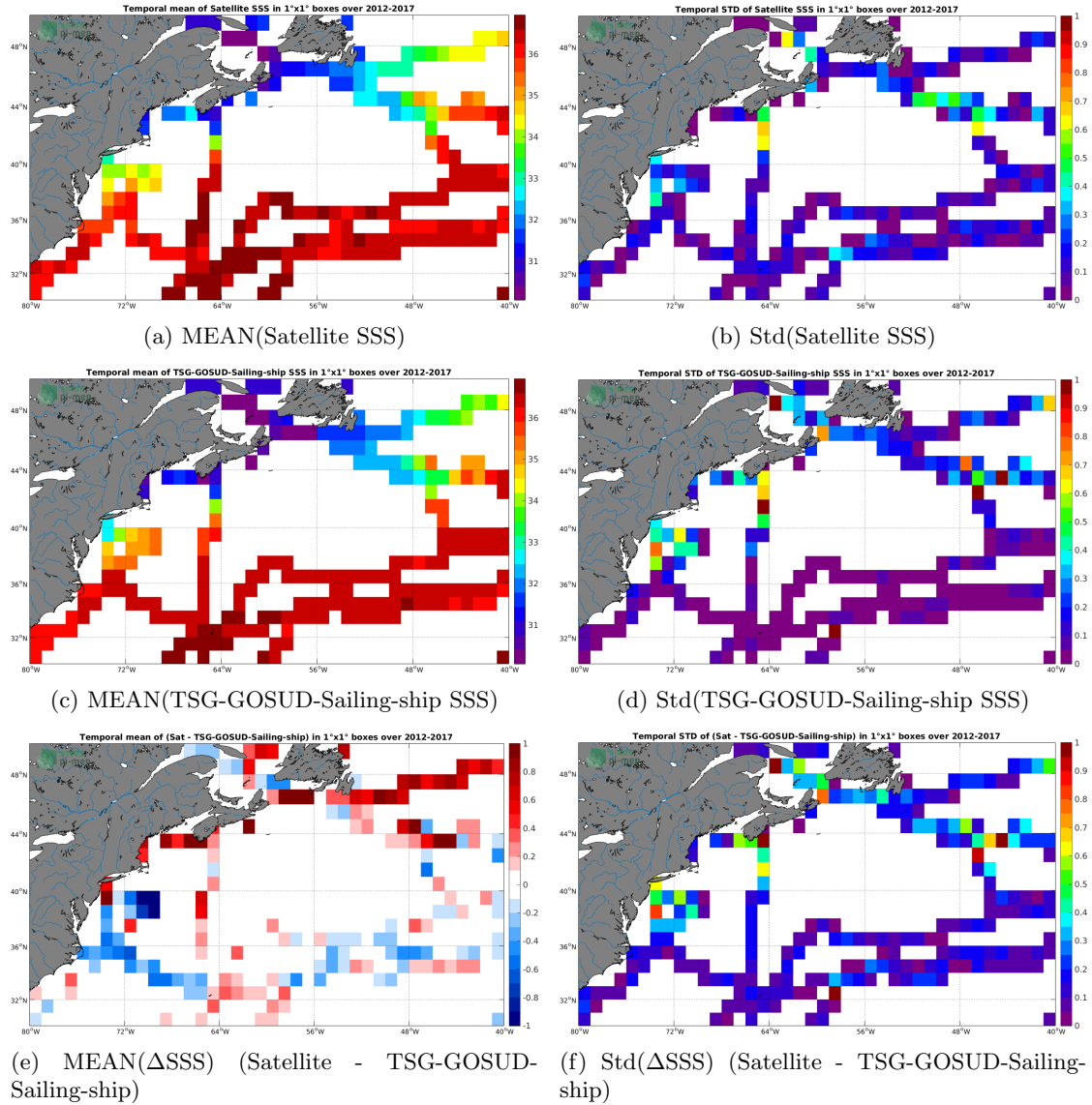
Figure 6: Temporal mean (left) and Std (right) of SSS from SMOS-L3-CATDS-CECOS-LOCEAN-V4-9DAYS-25KM (top), TSG-GOSUD-Sailing-ship (middle), and of \Delta SSS (Satellite - TSG-GOSUD-Sailing-ship). Only match-up pairs are used to generate these maps.
