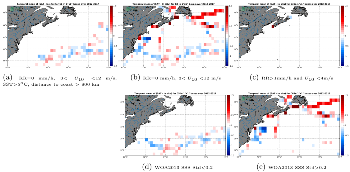
Figure 12: Temporal mean gridded over spatial boxes of size 1°x1° of \Delta SSS (SMOS-L3-CATDS-CECOS-LOCEAN-V4-9DAYS-25KM - TSG-GOSUD-Sailing-ship) for 5 different subdatasets corresponding to:RR=0 mm/h, 3 < U_{10} < 12 m/s, SST>5°C, distance to coast > 800 km (a), RR=0 mm/h, 3 < U_{10} < 12 m/s (b), RR>1mm/h and U_{10} < 4 m/s (c), WOA2013 SSS Std<0.2 (d), WOA2013 SSS Std>0.2 (e).
