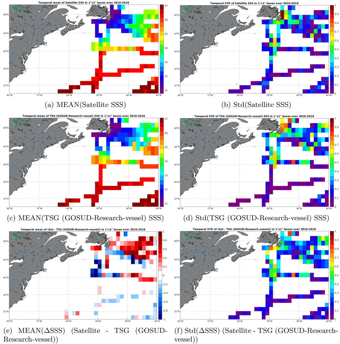
Figure 6: Temporal mean (left) and Std (right) of SSS from SMOS SSS L3 v4 - 9 Days (CATDS-CECOS-LOCEAN) (top), TSG (GOSUD-Research-vessel) (middle), and of \Delta SSS (Satellite - TSG (GOSUD-Research-vessel)). Only match-up pairs are used to generate these maps.
