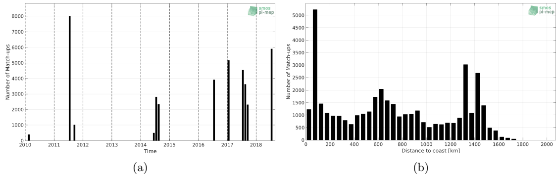
Figure 1: Number of match-ups between TSG (GOSUD-Research-vessel) and SMOS SSS L3 v4 - 9 Days (CATDS-CECOS-LOCEAN) SSS as a function of time (a) and as function of the distance to coast (b) over the Gulf Stream Pi-MEP region and for the full satellite product period.
