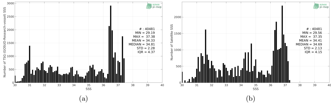
Figure 2: Histograms of SSS from TSG (GOSUD-Research-vessel) (a) and SMOS SSS L3 v4 - 9 Days (CATDS-CECOS-LOCEAN) (b) considering all match-up pairs per bins of 0.1 over the Gulf Stream Pi-MEP region and for the full satellite product period.
