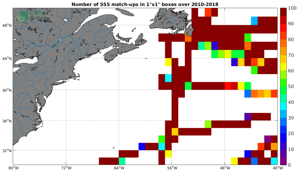
Figure 4: Number of SSS match-ups between TSG (GOSUD-Research-vessel) SSS and the SMOS SSS L3 v4 - 9 Days (CATDS-CECOS-LOCEAN) SSS product for the Gulf Stream Pi-MEP region over 1^\circ \times 1^\circ boxes and for the full satellite product period.
