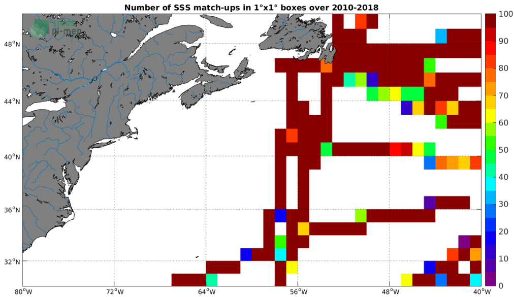
Figure 4: Number of SSS match-ups between TSG-GOSUD-Research-vessel SSS and the SMOS-L3-CATDS-CECOS-LOCEAN-V4-9DAYS-25KM SSS product for the Gulf Stream Pi-MEP region over 1°x1° boxes and for the full satellite product period.
