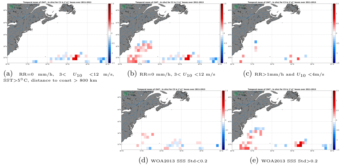
Figure 11: Temporal mean gridded over spatial boxes of size 1^{\circ}\times 1^{\circ} of \Delta\text{SSS} (SMOS SSS L3 v4 - 9 Days (CATDS-CECOS-LOCEAN) - Surface drifters) for 5 different subdatasets corresponding to:RR=0 mm/h, 3 < U_{10} < 12 m/s, SST >5^{\circ}\text{C} , distance to coast > 800 km (a), RR=0 mm/h, 3 < U_{10} < 12 m/s (b), RR >1 mm/h and U_{10} < 4 m/s (c), WOA2013 SSS Std <0.2 (d), WOA2013 SSS Std >0.2 (e).
