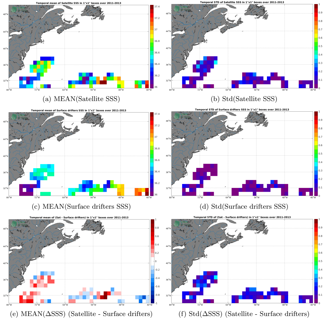
Figure 5: Temporal mean (left) and Std (right) of SSS from SMOS SSS L3 v4 - 9 Days (CATDS-CECOS-LOCEAN) (top), Surface drifters (middle), and of \Delta\text{SSS} (Satellite - Surface drifters). Only match-up pairs are used to generate these maps.
