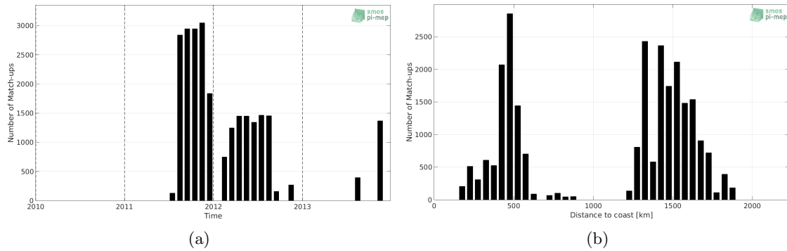
Figure 1: Number of match-ups between Surface drifters and SMOS SSS L3 v4 - 9 Days (CATDS-CECOS-LOCEAN) SSS as a function of time (a) and as function of the distance to coast (b) over the Gulf Stream Pi-MEP region and for the full satellite product period.
