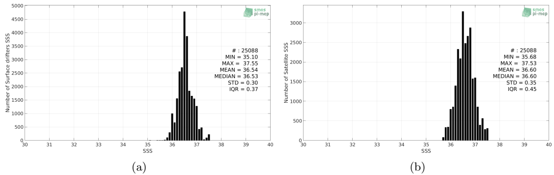
Figure 2: Histograms of SSS from Surface drifters (a) and SMOS SSS L3 v4 - 9 Days (CATDS-CECOS-LOCEAN) (b) considering all match-up pairs per bins of 0.1 over the Gulf Stream Pi-MEP region and for the full satellite product period.
