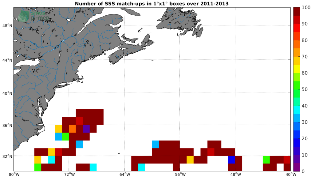
Figure 3: Number of SSS match-ups between Surface drifters SSS and the SMOS SSS L3 v4 - 9 Days (CATDS-CECOS-LOCEAN) SSS product for the Gulf Stream Pi-MEP region over 1^\circ \times 1^\circ boxes and for the full satellite product period.
