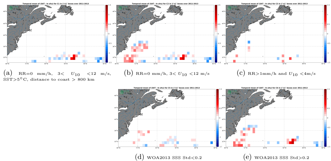
Figure 11: Temporal mean gridded over spatial boxes of size 1^{\circ}\times 1^{\circ} of \Delta\text{SSS} (SMOS-L3-CATDS-CECOS-LOCEAN-V4-9DAYS-25KM - Surface drifters) for 5 different subdatasets corresponding to:RR=0 mm/h, 3 < U_{10} < 12 m/s, SST >5^{\circ}\text{C} , distance to coast > 800 km (a), RR=0 mm/h, 3 < U_{10} < 12 m/s (b), RR >1 mm/h and U_{10} < 4 m/s (c), WOA2013 SSS Std <0.2 (d), WOA2013 SSS Std >0.2 (e).
