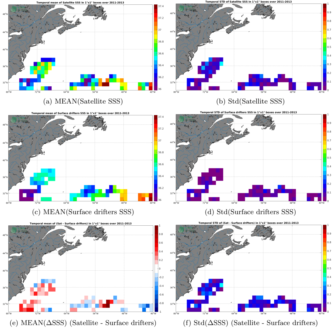
Figure 5: Temporal mean (left) and Std (right) of SSS from SMOS-L3-CATDS-CECOS-LOCEAN-V4-9DAYS-25KM (top), Surface drifters (middle), and of \Delta\text{SSS} (Satellite - Surface drifters). Only match-up pairs are used to generate these maps.
