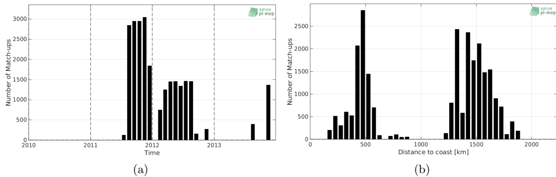
Figure 1: Number of match-ups between Surface drifters and SMOS-L3-CATDS-CECOS-LOCEAN-V4-9DAYS-25KM SSS as a function of time (a) and as function of the distance to coast (b) over the Gulf Stream Pi-MEP region and for the full satellite product period.
