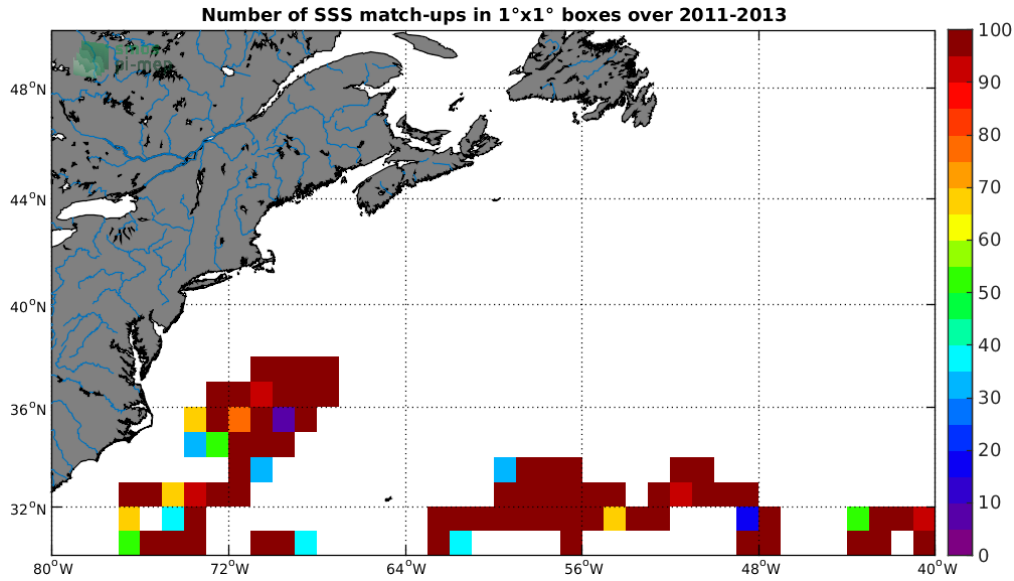
Figure 3: Number of SSS match-ups between Surface drifters SSS and the SMOS-L3-CATDS-CECOS-LOCEAN-V4-9DAYS-25KM SSS product for the Gulf Stream Pi-MEP region over 1^\circ \times 1^\circ boxes and for the full satellite product period.
