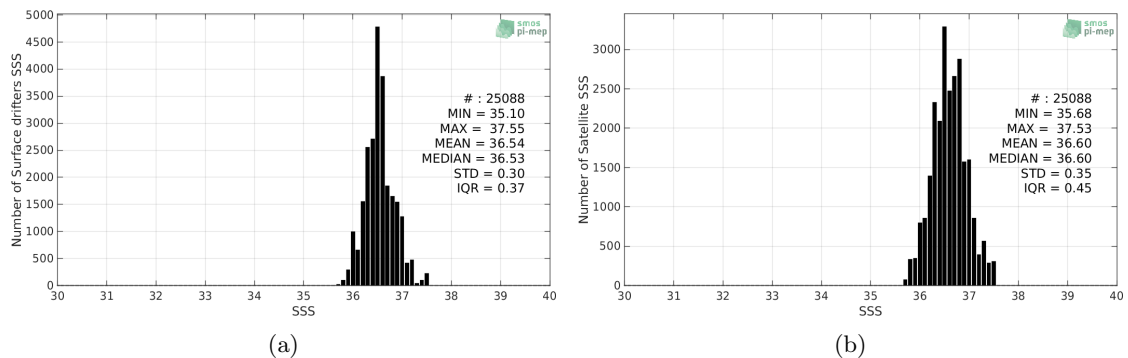
Figure 2: Histograms of SSS from Surface drifters (a) and SMOS-L3-CATDS-CECOS-LOCEAN-V4-9DAYS-25KM (b) considering all match-up pairs per bins of 0.1 over the Gulf Stream Pi-MEP region and for the full satellite product period.
