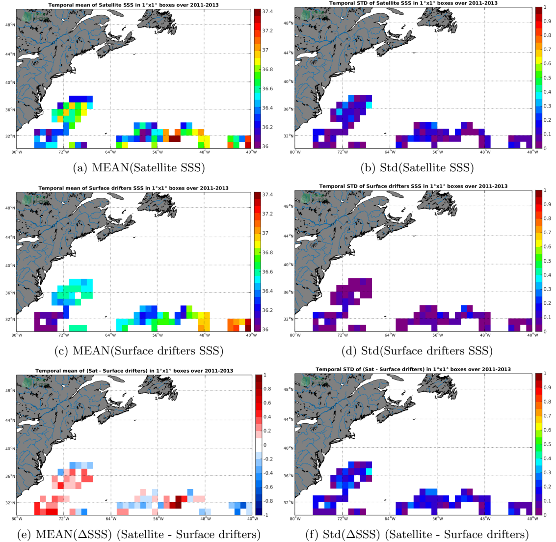
Figure 5: Temporal mean (left) and Std (right) of SSS from SMOS-L3-CATDS-CECOS-LOCEAN-V4-9DAYS-25KM (top), Surface drifters (middle), and of \Delta\text{SSS} (Satellite - Surface drifters). Only match-up pairs are used to generate these maps.
