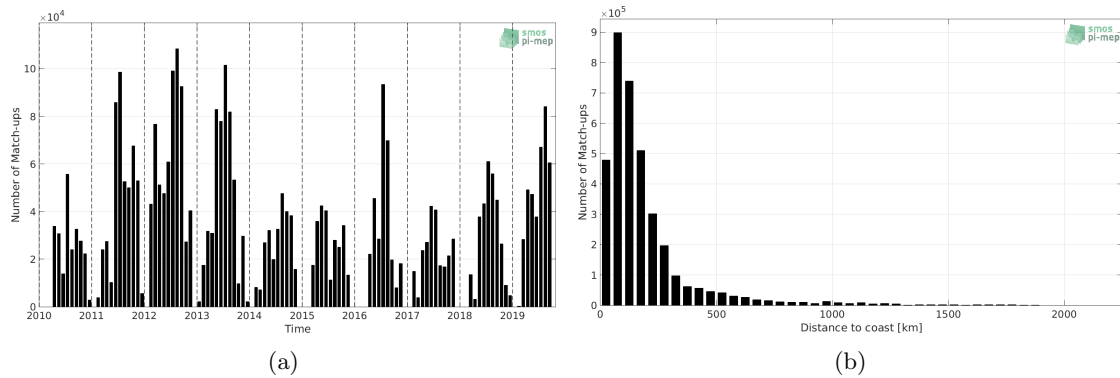
Figure 1: Number of match-ups between TSG (SAMOS) and SMOS SSS L3 v4 - 18 Days (CATDS-CECOS-LOCEAN) SSS as a function of time (a) and as function of the distance to coast (b) over the Gulf Stream Pi-MEP region and for the full satellite product period.
