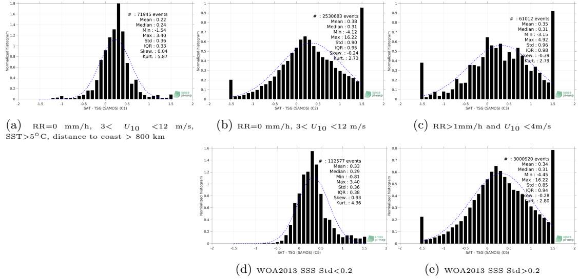
Figure 13: Normalized histogram of \Delta SSS (SMOS SSS L3 v4 - 18 Days (CATDS-CECOS-LOCEAN) - TSG (SAMOS)) for 5 different subdatasets corresponding to: RR=0 mm/h, 3 < U_{10} < 12 m/s, SST > 5°C, distance to coast > 800 km (a), RR=0 mm/h, 3 < U_{10} < 12 m/s (b), RR > 1mm/h and U_{10} < 4 m/s (c), WOA2013 SSS Std < 0.2 (d), WOA2013 SSS Std > 0.2 (e).
