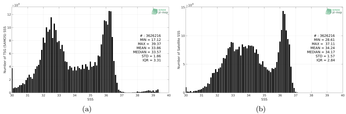
Figure 2: Histograms of SSS from TSG (SAMOS) (a) and SMOS SSS L3 v4 - 18 Days (CATDS-CECOS-LOCEAN) (b) considering all match-up pairs per bins of 0.1 over the Gulf Stream Pi-MEP region and for the full satellite product period.
