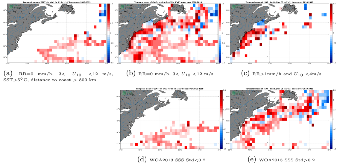
Figure 12: Temporal mean gridded over spatial boxes of size 1^{\circ}\times 1^{\circ} of \Delta\text{SSS} (SMOS SSS L3 v4 - 18 Days (CATDS-CECOS-LOCEAN) - TSG (SAMOS)) for 5 different subdatasets corresponding to:RR=0 mm/h, 3 < U_{10} < 12 m/s, SST >5^{\circ}\text{C} , distance to coast > 800 km (a), RR=0 mm/h, 3 < U_{10} < 12 m/s (b), RR >1 mm/h and U_{10} < 4 m/s (c), WOA2013 SSS Std <0.2 (d), WOA2013 SSS Std >0.2 (e).
