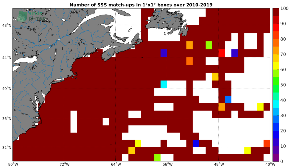
Figure 4: Number of SSS match-ups between TSG (SAMOS) SSS and the SMOS SSS L3 v4 - 18 Days (CATDS-CECOS-LOCEAN) SSS product for the Gulf Stream Pi-MEP region over 1^\circ \times 1^\circ boxes and for the full satellite product period.
