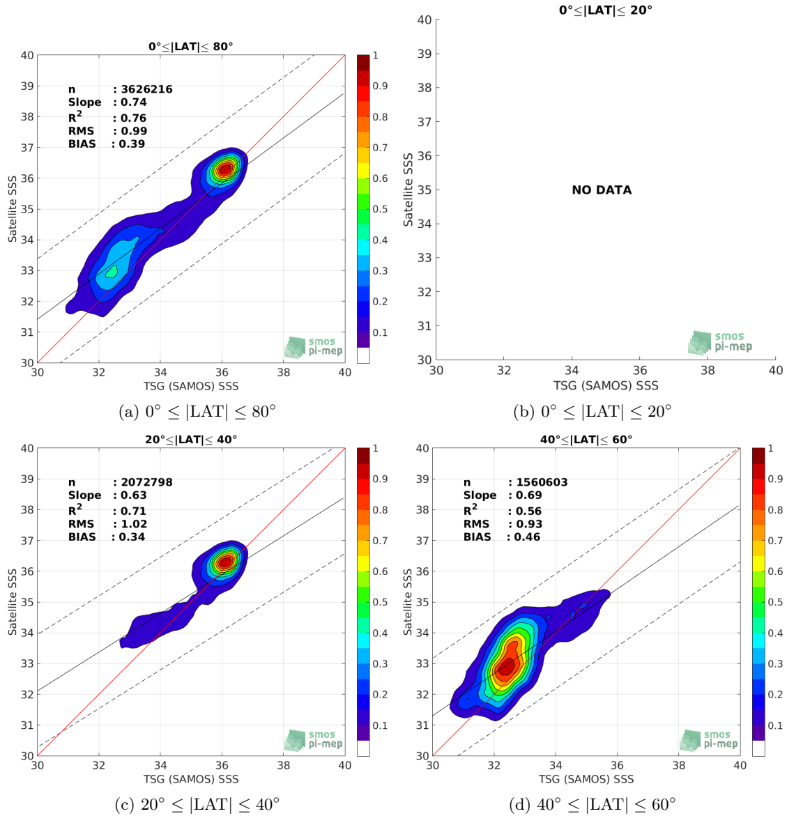
Figure 9: Contour maps of the concentration of SMOS SSS L3 v4 - 18 Days (CATDS-CECOS-LOCEAN) SSS ( y -axis) versus TSG (SAMOS) SSS ( x -axis) at match-up pairs for different latitude bands. For each plot, the red line shows x=y . The black thin and dashed lines indicate a linear fit through the data cloud and the \pm 95\% confidence levels, respectively. The number match-up pairs n , the slope and R^2 coefficient of the linear fit, the root mean square (RMS) and the mean bias between satellite and in situ data are indicated for each latitude band in each plots.
