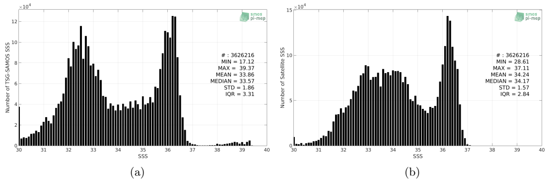
Figure 2: Histograms of SSS from TSG-SAMOS (a) and SMOS-L3-CATDS-CECOS-LOCEAN-V4-18DAYS-25KM (b) considering all match-up pairs per bins of 0.1 over the Gulf Stream Pi-MEP region and for the full satellite product period.
