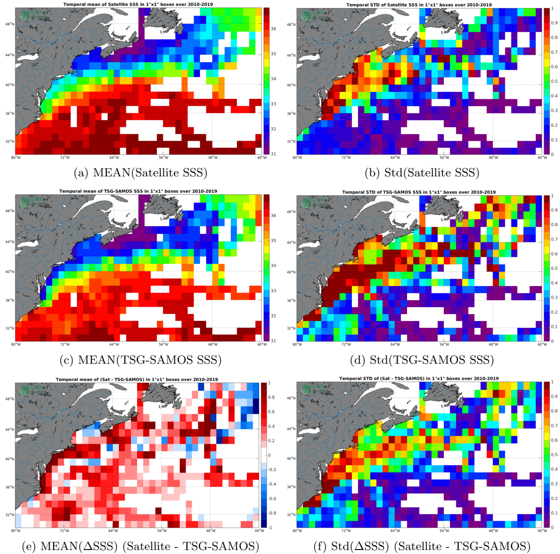
Figure 6: Temporal mean (left) and Std (right) of SSS from SMOS-L3-CATDS-CECOS-LOCEAN-V4-18DAYS-25KM (top), TSG-SAMOS (middle), and of \Delta SSS (Satellite - TSG-SAMOS). Only match-up pairs are used to generate these maps.
