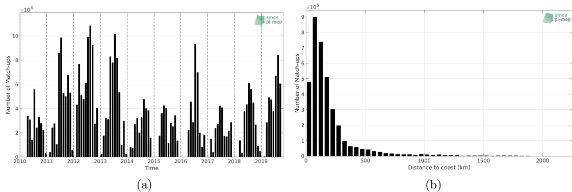
Figure 1: Number of match-ups between TSG-SAMOS and SMOS-L3-CATDS-CECOS-LOCEAN-V4-18DAYS-25KM SSS as a function of time (a) and as function of the distance to coast (b) over the Gulf Stream Pi-MEP region and for the full satellite product period.
