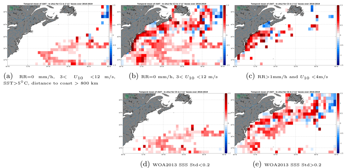
Figure 12: Temporal mean gridded over spatial boxes of size 1^{\circ}\times 1^{\circ} of \Delta\text{SSS} (SMOS-L3-CATDS-CECOS-LOCEAN-V4-18DAYS-25KM - TSG-SAMOS) for 5 different subdatasets corresponding to:RR=0 mm/h, 3 < U_{10} < 12 m/s, SST >5^{\circ}\text{C} , distance to coast > 800 km (a), RR=0 mm/h, 3 < U_{10} < 12 m/s (b), RR >1 mm/h and U_{10} < 4 m/s (c), WOA2013 SSS Std <0.2 (d), WOA2013 SSS Std >0.2 (e).
