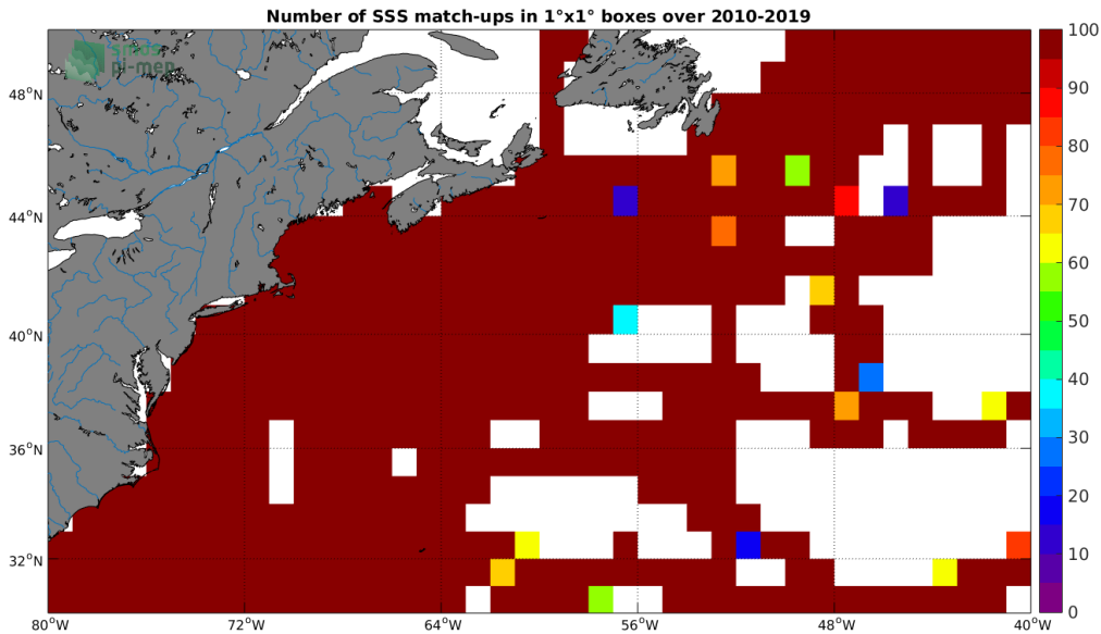
Figure 4: Number of SSS match-ups between TSG-SAMOS SSS and the SMOS-L3-CATDS-CECOS-LOCEAN-V4-18DAYS-25KM SSS product for the Gulf Stream Pi-MEP region over 1^\circ \times 1^\circ boxes and for the full satellite product period.
