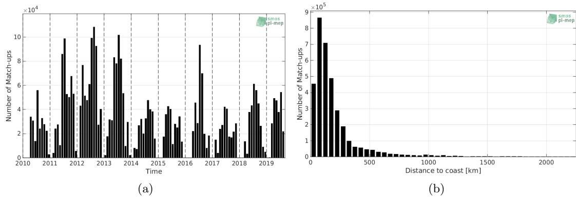
Figure 1: Number of match-ups between TSG-SAMOS and SMOS-L3-CATDS-CECOS-LOCEAN-V4-18DAYS-25KM SSS as a function of time (a) and as function of the distance to coast (b) over the Gulf Stream Pi-MEP region and for the full satellite product period.
