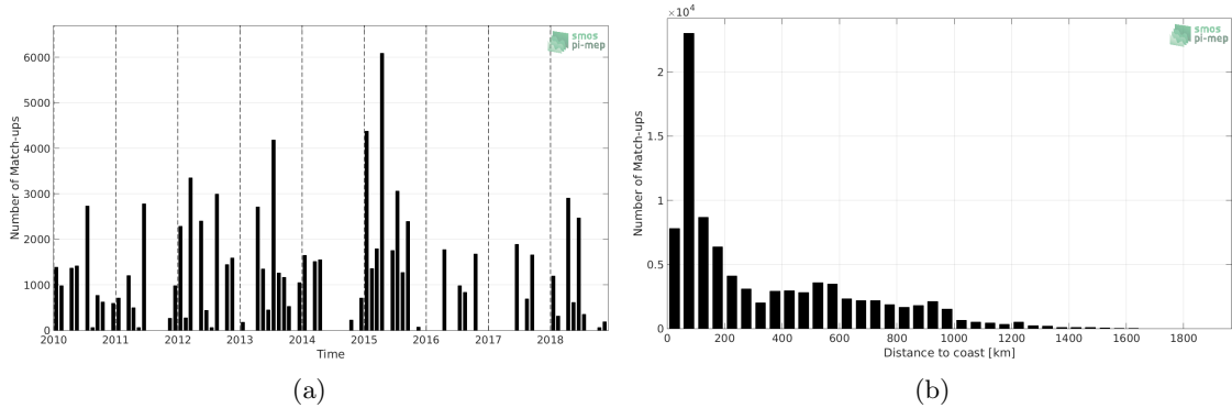
Figure 1: Number of match-ups between TSG-LEGOS-DM and SMOS-L3-CATDS-CECOS-LOCEAN-V4-18DAYS-25KM SSS as a function of time (a) and as function of the distance to coast (b) over the Gulf Stream Pi-MEP region and for the full satellite product period.
