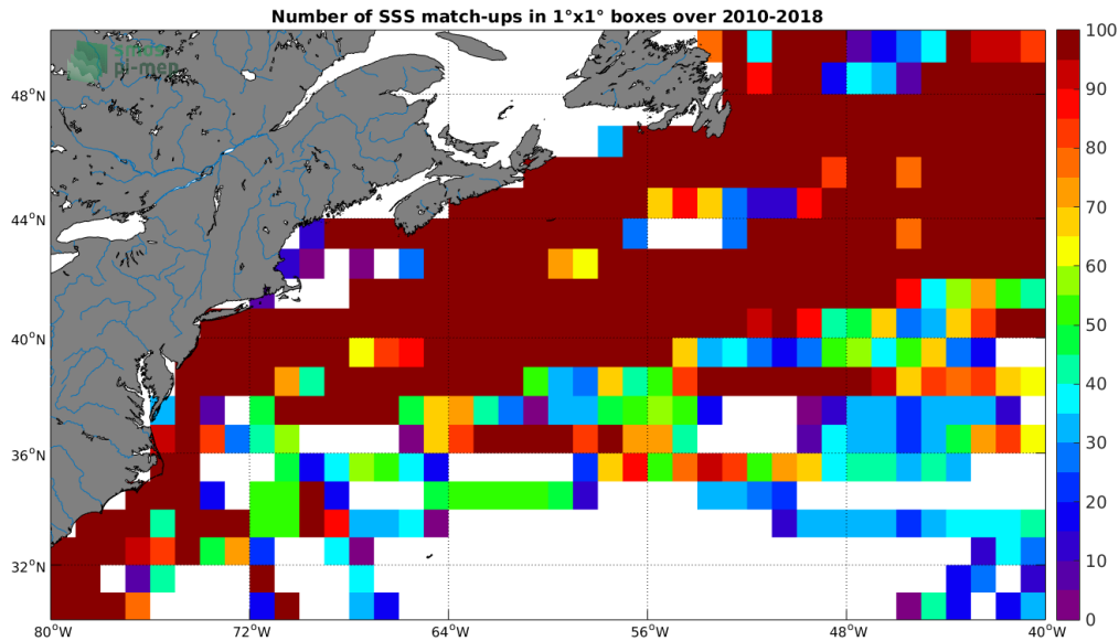
Figure 4: Number of SSS match-ups between TSG-LEGOS-DM SSS and the SMOS-L3-CATDS-CECOS-LOCEAN-V4-18DAYS-25KM SSS product for the Gulf Stream Pi-MEP region over 1^\circ \times 1^\circ boxes and for the full satellite product period.
