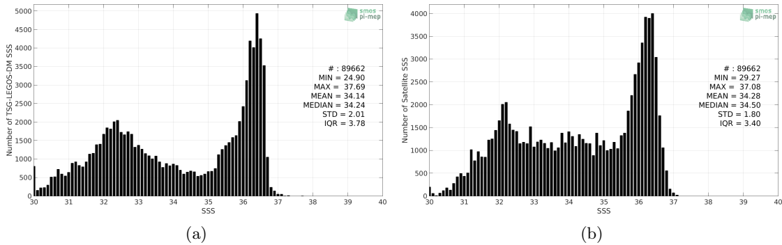
Figure 2: Histograms of SSS from TSG-LEGOS-DM (a) and SMOS-L3-CATDS-CECOS-LOCEAN-V4-18DAYS-25KM (b) considering all match-up pairs per bins of 0.1 over the Gulf Stream Pi-MEP region and for the full satellite product period.
