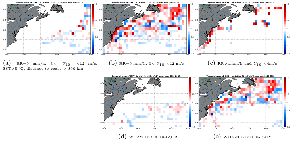
Figure 12: Temporal mean gridded over spatial boxes of size 1^\circ \times 1^\circ of \Delta SSS (SMOS-L3-CATDS-CECOS-LOCEAN-V4-18DAYS-25KM - TSG-LEGOS-DM) for 5 different subdatasets corresponding to:RR=0 mm/h, 3 < U_{10} < 12 m/s, SST >5^\circ C, distance to coast > 800 km (a), RR=0 mm/h, 3 < U_{10} < 12 m/s (b), RR >1 mm/h and U_{10} < 4 m/s (c), WOA2013 SSS Std <0.2 (d), WOA2013 SSS Std >0.2 (e).
