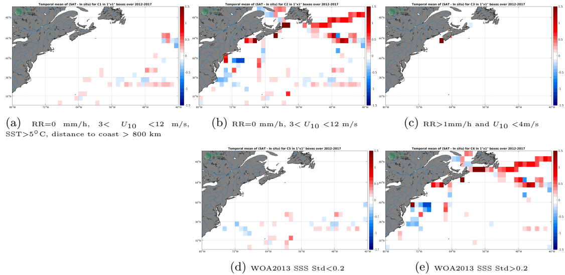
Figure 12: Temporal mean gridded over spatial boxes of size 1^\circ \times 1^\circ of \Delta SSS (SMOS SSS L3 v4 - 18 Days (CATDS-CECOS-LOCEAN) - TSG (GOSUD-Sailing-ship)) for 5 different subdatasets corresponding to: RR=0 mm/h, 3 < U_{10} < 12 m/s, SST > 5^\circ\text{C} , distance to coast > 800 km (a), RR=0 mm/h, 3 < U_{10} < 12 m/s (b), RR > 1 mm/h and U_{10} < 4 m/s (c), WOA2013 SSS Std < 0.2 (d), WOA2013 SSS Std > 0.2 (e).
