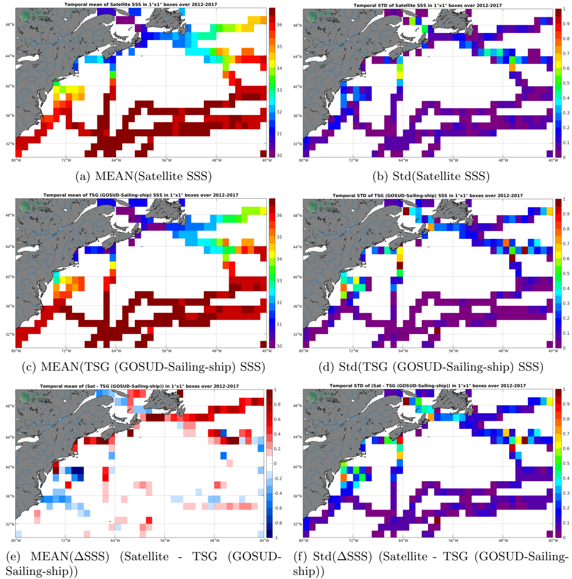
Figure 6: Temporal mean (left) and Std (right) of SSS from SMOS SSS L3 v4 - 18 Days (CATDS-CECOS-LOCEAN) (top), TSG (GOSUD-Sailing-ship) (middle), and of \Delta SSS (Satellite - TSG (GOSUD-Sailing-ship)). Only match-up pairs are used to generate these maps.
