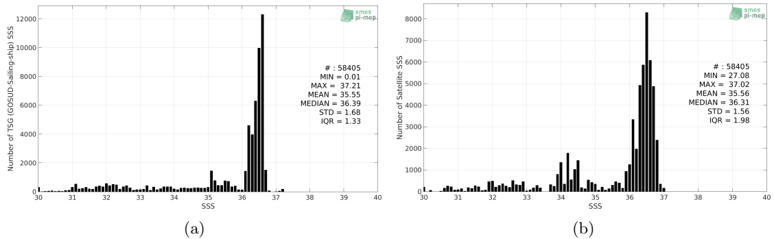
Figure 2: Histograms of SSS from TSG (GOSUD-Sailing-ship) (a) and SMOS SSS L3 v4 - 18 Days (CATDS-CECOS-LOCEAN) (b) considering all match-up pairs per bins of 0.1 over the Gulf Stream Pi-MEP region and for the full satellite product period.
