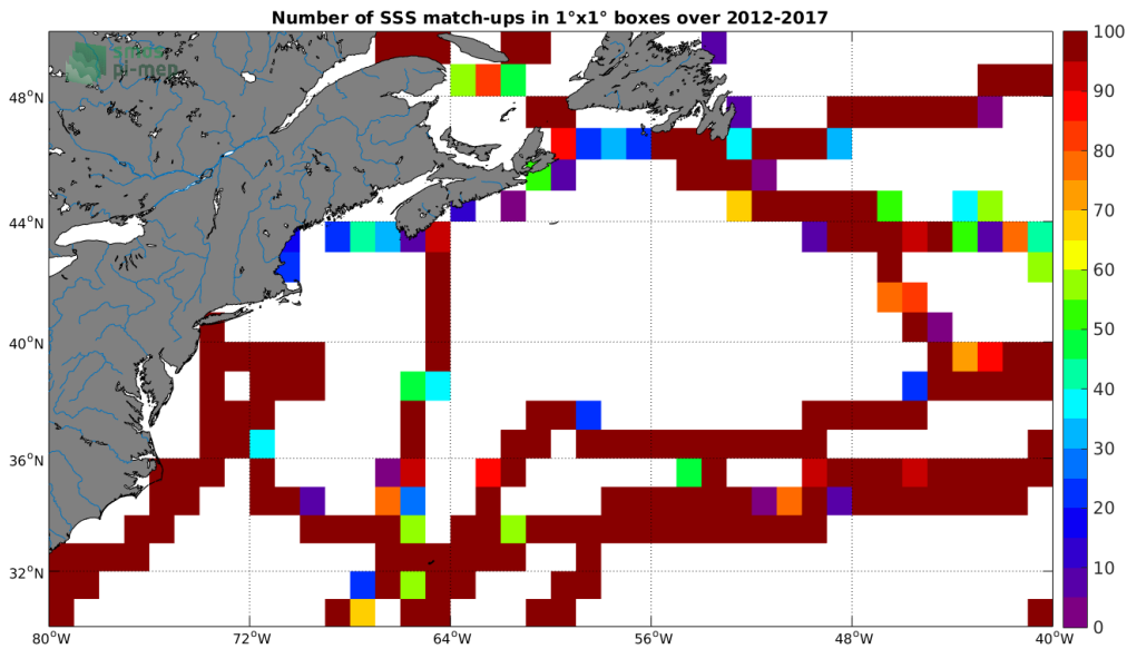
Figure 4: Number of SSS match-ups between TSG (GOSUD-Sailing-ship) SSS and the SMOS SSS L3 v4 - 18 Days (CATDS-CECOS-LOCEAN) SSS product for the Gulf Stream Pi-MEP region over 1^\circ \times 1^\circ boxes and for the full satellite product period.
