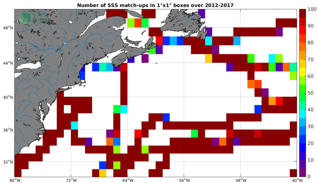
Figure 4: Number of SSS match-ups between TSG-GOSUD-Sailing-ship SSS and the SMOS-L3-CATDS-CECOS-LOCEAN-V4-18DAYS-25KM SSS product for the Gulf Stream Pi-MEP region over 1^\circ \times 1^\circ boxes and for the full satellite product period.
