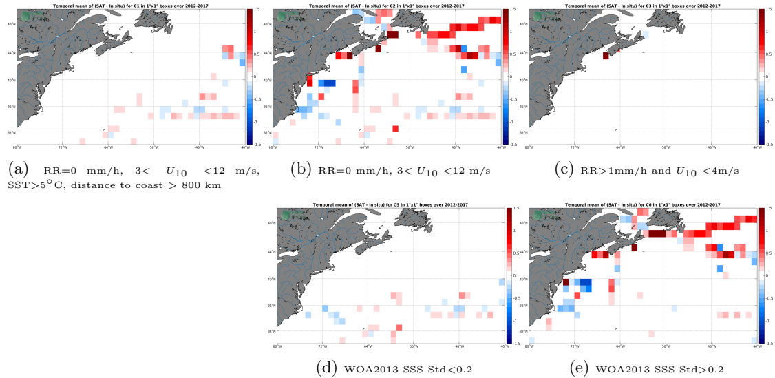
Figure 12: Temporal mean gridded over spatial boxes of size 1^{\circ}\times 1^{\circ} of \Delta SSS (SMOS-L3-CATDS-CECOS-LOCEAN-V4-18DAYS-25KM - TSG-GOSUD-Sailing-ship) for 5 different subdatasets corresponding to:RR=0 mm/h, 3 < U_{10} < 12 m/s, SST >5^{\circ}\text{C} , distance to coast > 800 km (a), RR=0 mm/h, 3 < U_{10} < 12 m/s (b), RR >1 mm/h and U_{10} < 4 m/s (c), WOA2013 SSS Std <0.2 (d), WOA2013 SSS Std >0.2 (e).
