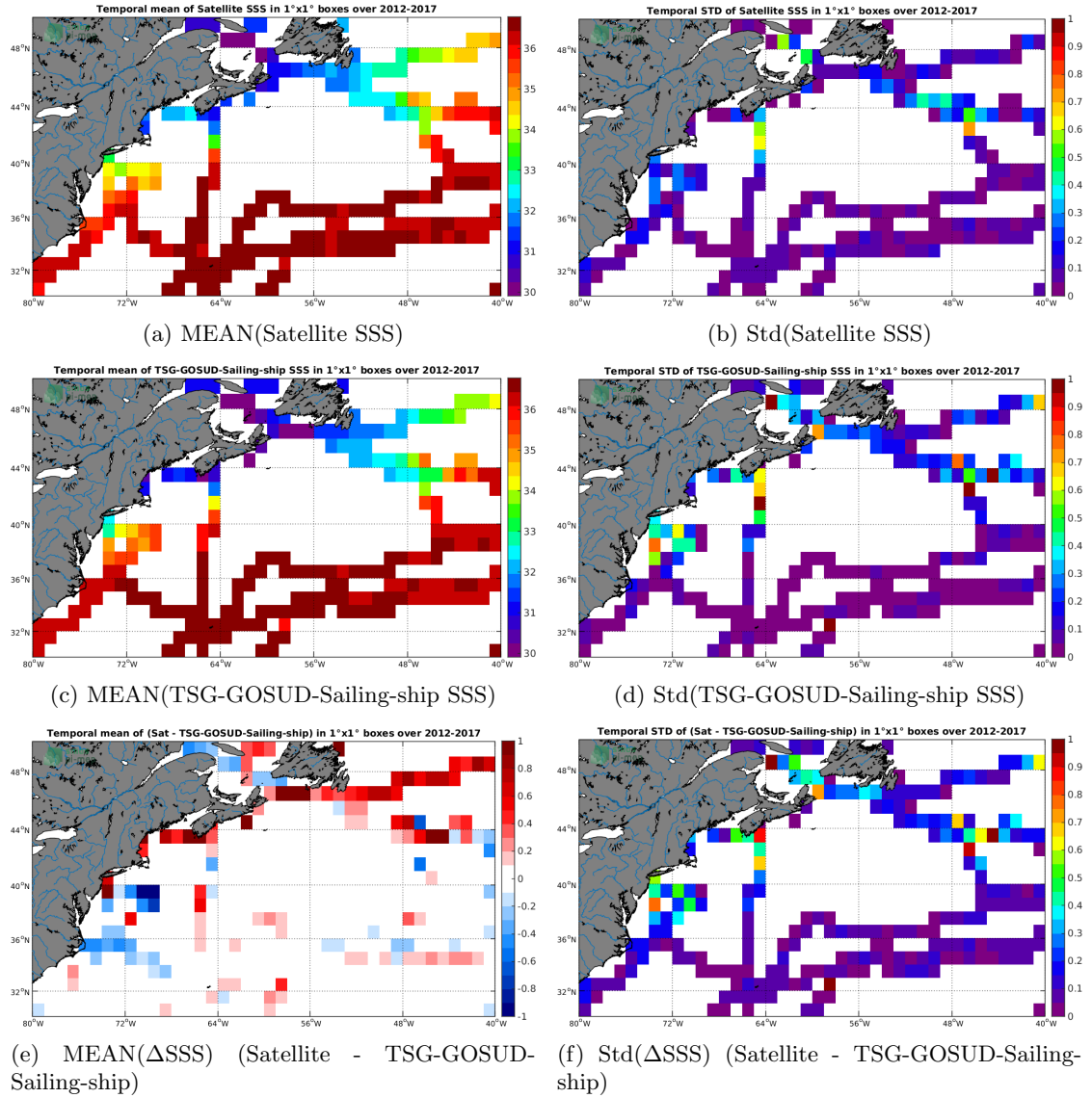
Figure 6: Temporal mean (left) and Std (right) of SSS from SMOS-L3-CATDS-CECOS-LOCEAN-V4-18DAYS-25KM (top), TSG-GOSUD-Sailing-ship (middle), and of \Delta SSS (Satellite - TSG-GOSUD-Sailing-ship). Only match-up pairs are used to generate these maps.
