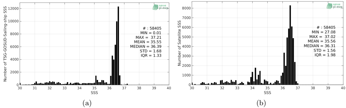
Figure 2: Histograms of SSS from TSG-GOSUD-Sailing-ship (a) and SMOS-L3-CATDS-CECOS-LOCEAN-V4-18DAYS-25KM (b) considering all match-up pairs per bins of 0.1 over the Gulf Stream Pi-MEP region and for the full satellite product period.
