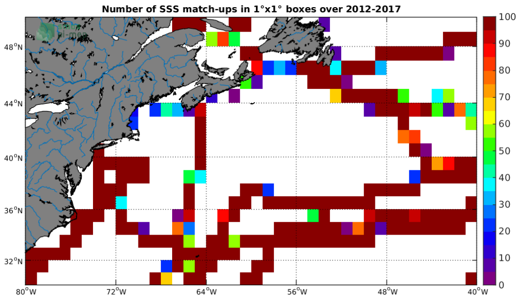
Figure 4: Number of SSS match-ups between TSG-GOSUD-Sailing-ship SSS and the SMOS-L3-CATDS-CECOS-LOCEAN-V4-18DAYS-25KM SSS product for the Gulf Stream Pi-MEP region over 1°x1° boxes and for the full satellite product period.
