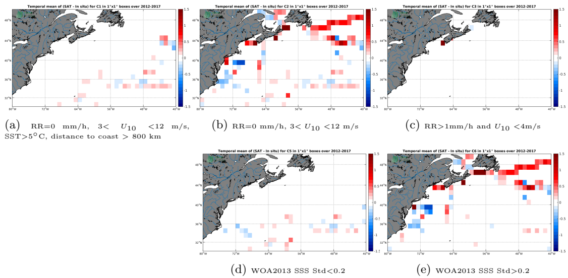
Figure 12: Temporal mean gridded over spatial boxes of size 1°x1° of \Delta SSS (SMOS-L3-CATDS-CECOS-LOCEAN-V4-18DAYS-25KM - TSG-GOSUD-Sailing-ship) for 5 different subdatasets corresponding to:RR=0 mm/h, 3 < U_{10} < 12 m/s, SST>5°C, distance to coast > 800 km (a), RR=0 mm/h, 3 < U_{10} < 12 m/s (b), RR>1mm/h and U_{10} < 4 m/s (c), WOA2013 SSS Std<0.2 (d), WOA2013 SSS Std>0.2 (e).
