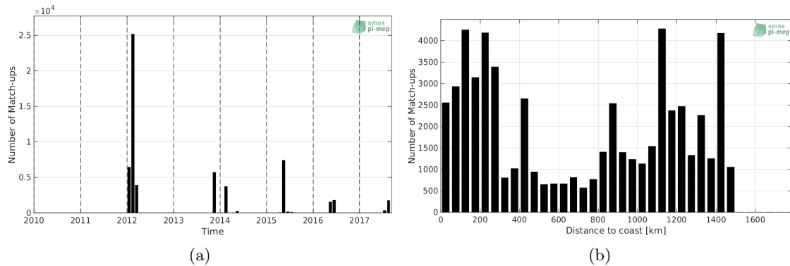
Figure 1: Number of match-ups between TSG-GOSUD-Sailing-ship and SMOS-L3-CATDS-CECOS-LOCEAN-V4-18DAYS-25KM SSS as a function of time (a) and as function of the distance to coast (b) over the Gulf Stream Pi-MEP region and for the full satellite product period.
