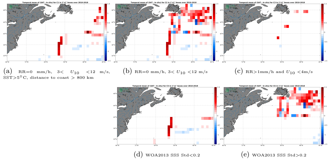
Figure 12: Temporal mean gridded over spatial boxes of size 1^{\circ}\times 1^{\circ} of \Delta SSS (SMOS-L3-CATDS-CECOS-LOCEAN-V4-18DAYS-25KM - TSG-GOSUD-Research-vessel) for 5 different subdatasets corresponding to:RR=0 mm/h, 3 < U_{10} < 12 m/s, SST >5^{\circ}\text{C} , distance to coast > 800 km (a), RR=0 mm/h, 3 < U_{10} < 12 m/s (b), RR >1 mm/h and U_{10} < 4 m/s (c), WOA2013 SSS Std <0.2 (d), WOA2013 SSS Std >0.2 (e).
