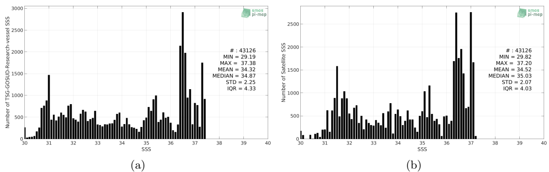
Figure 2: Histograms of SSS from TSG-GOSUD-Research-vessel (a) and SMOS-L3-CATDS-CECOS-LOCEAN-V4-18DAYS-25KM (b) considering all match-up pairs per bins of 0.1 over the Gulf Stream Pi-MEP region and for the full satellite product period.
