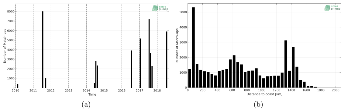
Figure 1: Number of match-ups between TSG-GOSUD-Research-vessel and SMOS-L3-CATDS-CECOS-LOCEAN-V4-18DAYS-25KM SSS as a function of time (a) and as function of the distance to coast (b) over the Gulf Stream Pi-MEP region and for the full satellite product period.
