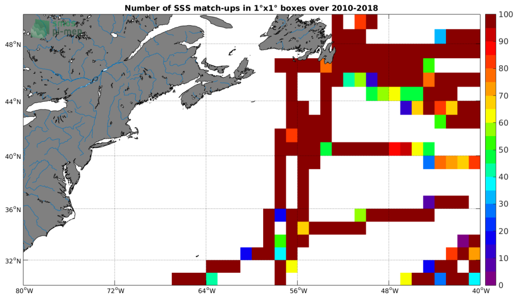
Figure 4: Number of SSS match-ups between TSG-GOSUD-Research-vessel SSS and the SMOS-L3-CATDS-CECOS-LOCEAN-V4-18DAYS-25KM SSS product for the Gulf Stream Pi-MEP region over 1^\circ \times 1^\circ boxes and for the full satellite product period.
