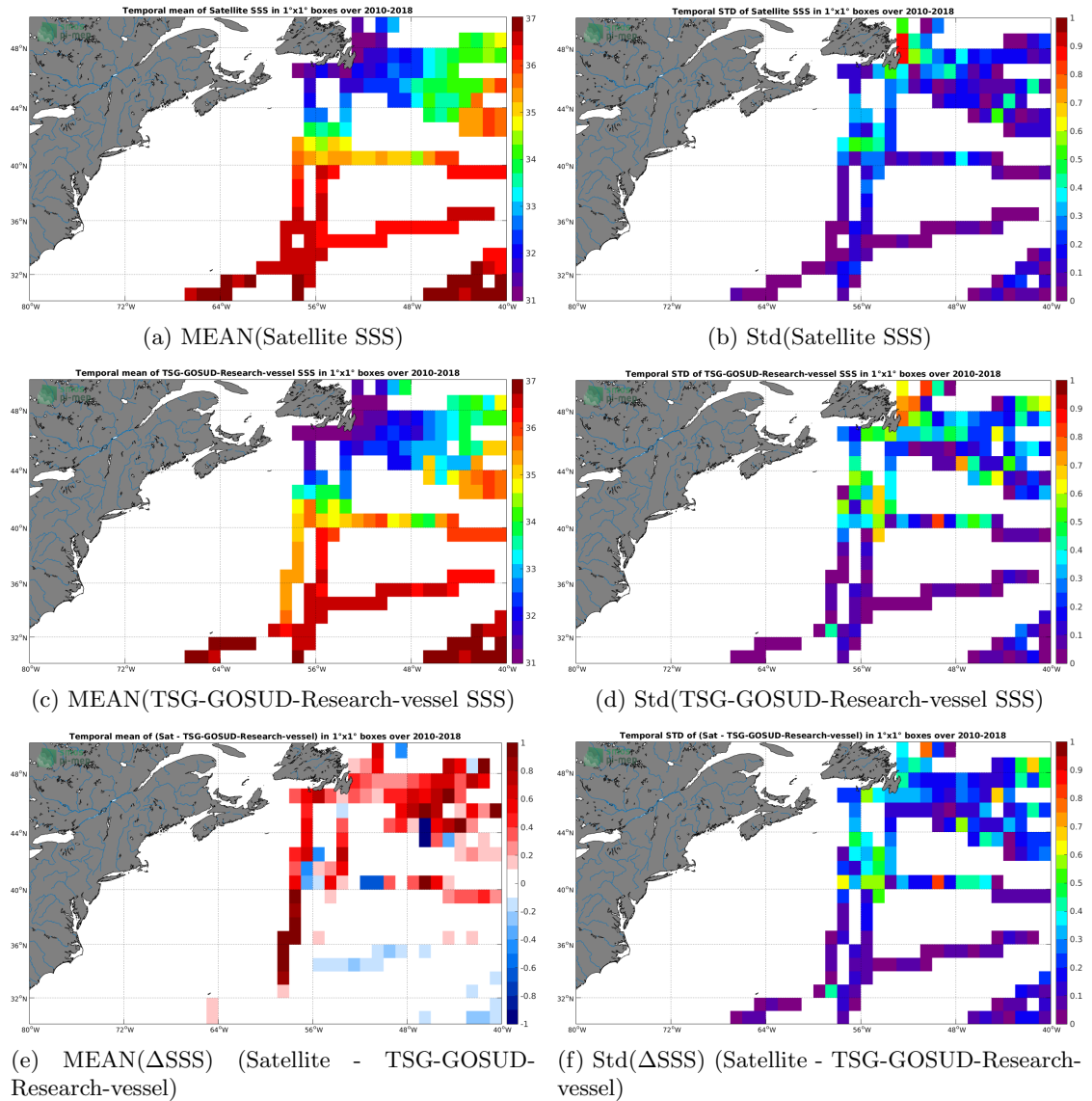
Figure 6: Temporal mean (left) and Std (right) of SSS from SMOS-L3-CATDS-CECOS-LOCEAN-V4-18DAYS-25KM (top), TSG-GOSUD-Research-vessel (middle), and of \Delta SSS (Satellite - TSG-GOSUD-Research-vessel). Only match-up pairs are used to generate these maps.
