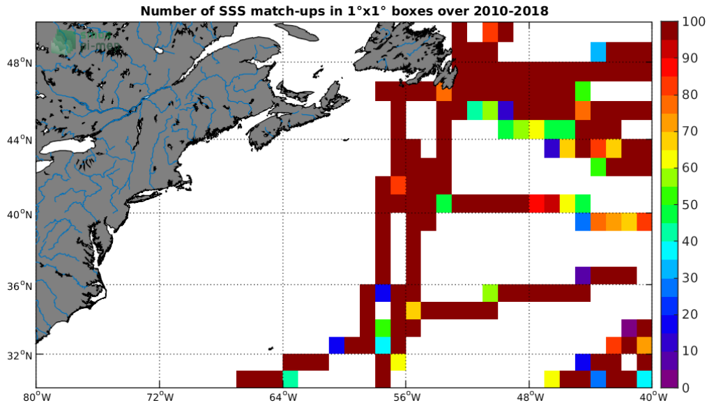
Figure 4: Number of SSS match-ups between TSG-GOSUD-Research-vessel SSS and the SMOS-L3-CATDS-CECOS-LOCEAN-V4-18DAYS-25KM SSS product for the Gulf Stream Pi-MEP region over 1°x1° boxes and for the full satellite product period.
