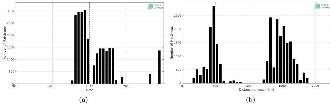
Figure 1: Number of match-ups between Surface drifters and SMOS SSS L3 v4 - 18 Days (CATDS-CECOS-LOCEAN) SSS as a function of time (a) and as function of the distance to coast (b) over the Gulf Stream Pi-MEP region and for the full satellite product period.
