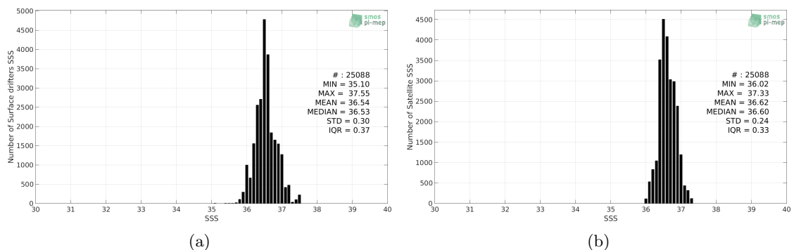
Figure 2: Histograms of SSS from Surface drifters (a) and SMOS SSS L3 v4 - 18 Days (CATDS-CECOS-LOCEAN) (b) considering all match-up pairs per bins of 0.1 over the Gulf Stream Pi-MEP region and for the full satellite product period.
