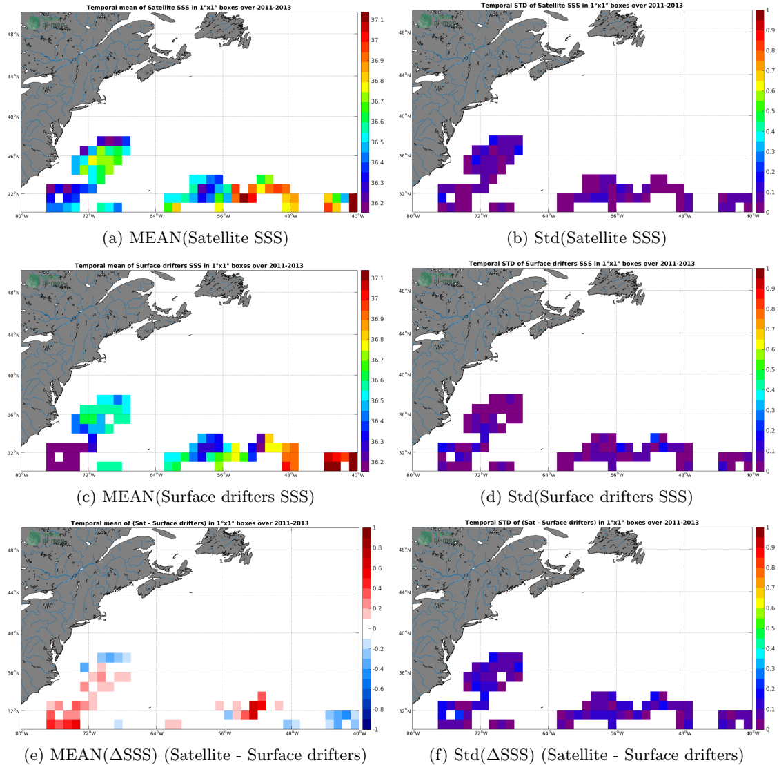
Figure 5: Temporal mean (left) and Std (right) of SSS from SMOS SSS L3 v4 - 18 Days (CATDS-CECOS-LOCEAN) (top), Surface drifters (middle), and of \Delta\text{SSS} (Satellite - Surface drifters). Only match-up pairs are used to generate these maps.
