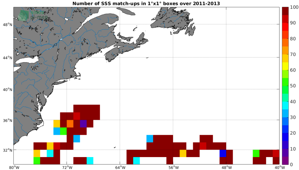
Figure 3: Number of SSS match-ups between Surface drifters SSS and the SMOS SSS L3 v4 - 18 Days (CATDS-CECOS-LOCEAN) SSS product for the Gulf Stream Pi-MEP region over 1^\circ \times 1^\circ boxes and for the full satellite product period.
