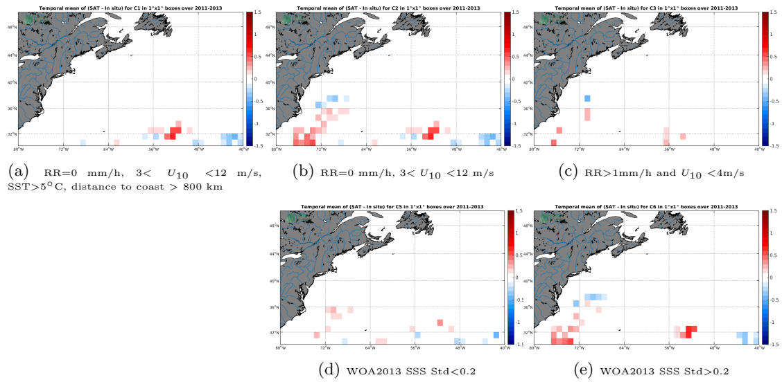
Figure 11: Temporal mean gridded over spatial boxes of size 1^\circ \times 1^\circ of \Delta SSS (SMOS-L3-CATDS-CECOS-LOCEAN-V4-18DAYS-25KM - Surface drifters) for 5 different subdatasets corresponding to:RR=0 mm/h, 3 < U_{10} < 12 m/s, SST >5^\circ\text{C} , distance to coast > 800 km (a), RR=0 mm/h, 3 < U_{10} < 12 m/s (b), RR >1 mm/h and U_{10} < 4 m/s (c), WOA2013 SSS Std <0.2 (d), WOA2013 SSS Std >0.2 (e).
