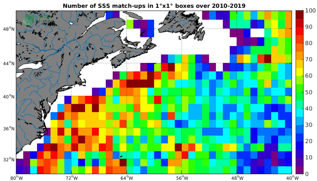
Figure 4: Number of SSS match-ups between Argo SSS and the SMOS-L3-CATDS-CECOS-LOCEAN-V4-18DAYS-25KM SSS product for the Gulf Stream Pi-MEP region over 1^\circ \times 1^\circ boxes and for the full satellite product period.
