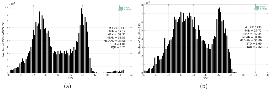
Figure 2: Histograms of SSS from TSG-SAMOS (a) and SMOS-L3-CATDS-CECOS-LOCEAN-V3-9DAYS-25KM (b) considering all match-up pairs per bins of 0.1 over the Gulf Stream Pi-MEP region and for the full satellite product period.
