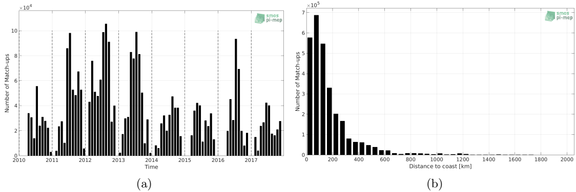
Figure 1: Number of match-ups between TSG-SAMOS and SMOS-L3-CATDS-CECOS-LOCEAN-V3-9DAYS-25KM SSS as a function of time (a) and as function of the distance to coast (b) over the Gulf Stream Pi-MEP region and for the full satellite product period.
