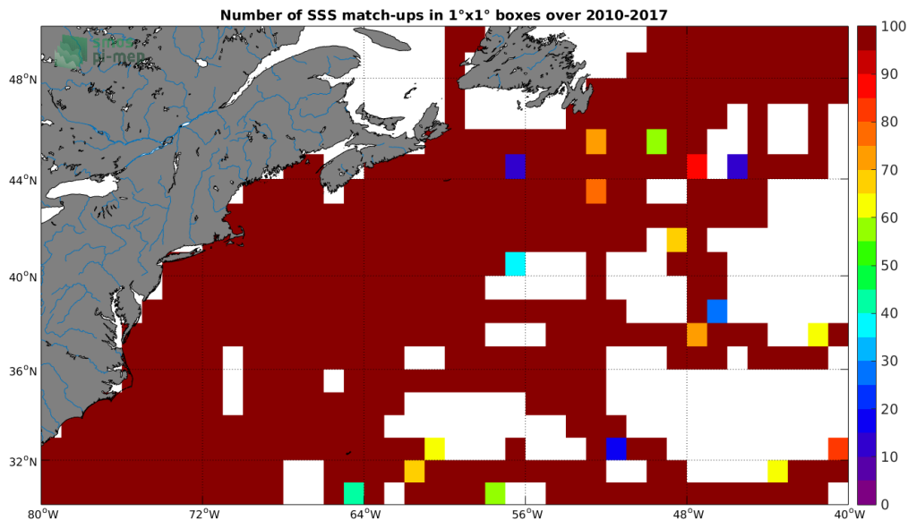
Figure 4: Number of SSS match-ups between TSG-SAMOS SSS and the SMOS-L3-CATDS-CECOS-LOCEAN-V3-9DAYS-25KM SSS product for the Gulf Stream Pi-MEP region over 1^\circ \times 1^\circ boxes and for the full satellite product period.
