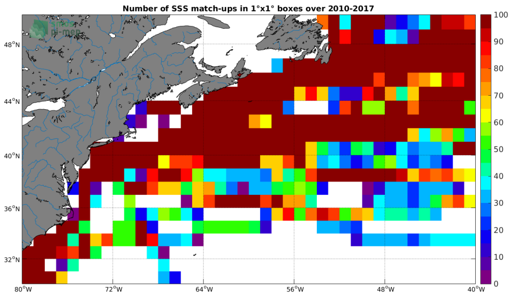
Figure 4: Number of SSS match-ups between TSG-LEGOS-DM SSS and the SMOS-L3-CATDS-CECOS-LOCEAN-V3-9DAYS-25KM SSS product for the Gulf Stream Pi-MEP region over 1^\circ \times 1^\circ boxes and for the full satellite product period.
