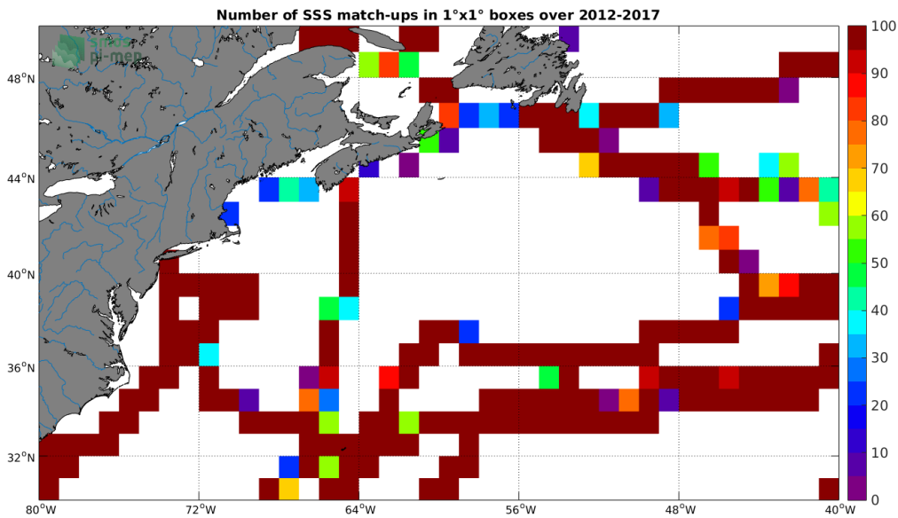
Figure 4: Number of SSS match-ups between TSG-GOSUD-Sailing-ship SSS and the SMOS-L3-CATDS-CECOS-LOCEAN-V3-9DAYS-25KM SSS product for the Gulf Stream Pi-MEP region over 1^\circ \times 1^\circ boxes and for the full satellite product period.
