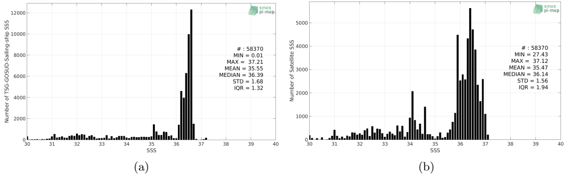
Figure 2: Histograms of SSS from TSG-GOSUD-Sailing-ship (a) and SMOS-L3-CATDS-CECOS-LOCEAN-V3-9DAYS-25KM (b) considering all match-up pairs per bins of 0.1 over the Gulf Stream Pi-MEP region and for the full satellite product period.
