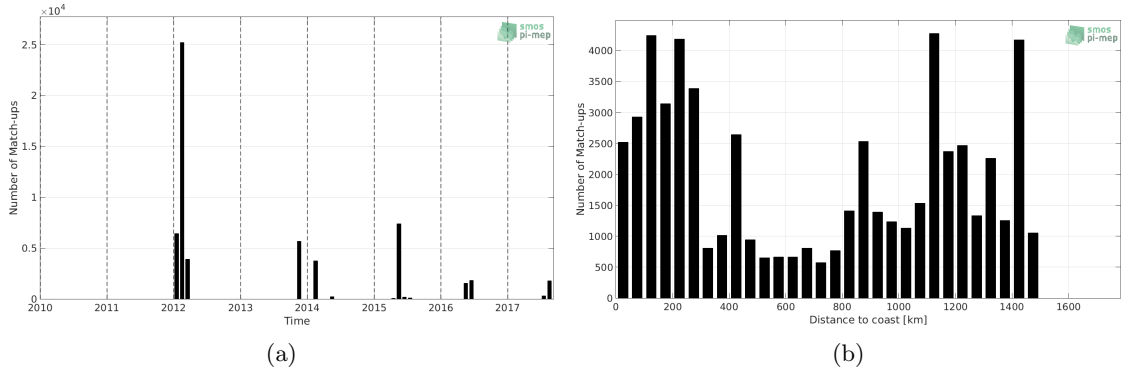
Figure 1: Number of match-ups between TSG-GOSUD-Sailing-ship and SMOS-L3-CATDS-CECOS-LOCEAN-V3-9DAYS-25KM SSS as a function of time (a) and as function of the distance to coast (b) over the Gulf Stream Pi-MEP region and for the full satellite product period.
