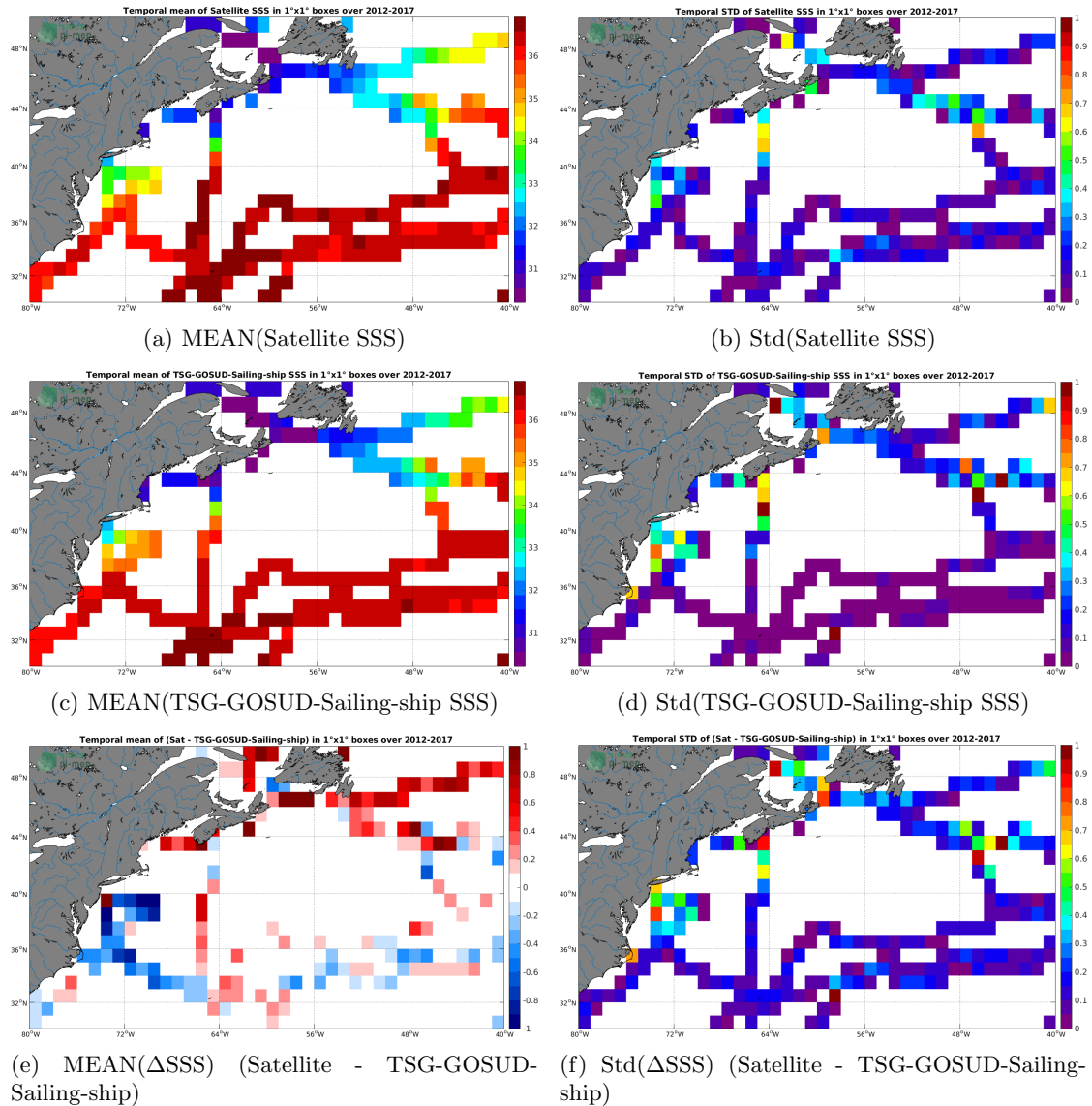
Figure 6: Temporal mean (left) and Std (right) of SSS from SMOS-L3-CATDS-CECOS-LOCEAN-V3-9DAYS-25KM (top), TSG-GOSUD-Sailing-ship (middle), and of \Delta SSS (Satellite - TSG-GOSUD-Sailing-ship). Only match-up pairs are used to generate these maps.
