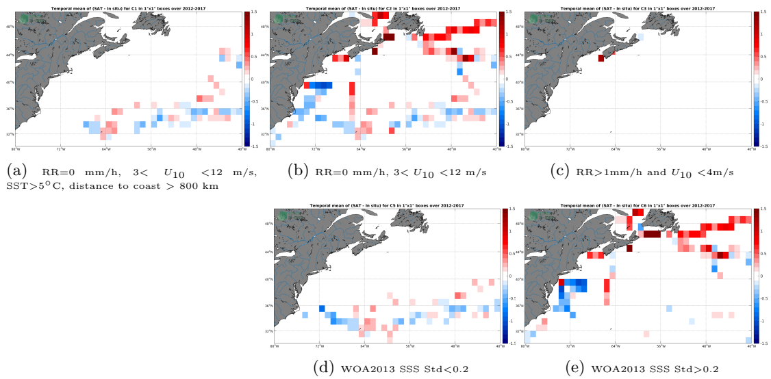
Figure 12: Temporal mean gridded over spatial boxes of size 1^\circ \times 1^\circ of \Delta SSS (SMOS-L3-CATDS-CECOS-LOCEAN-V3-9DAYS-25KM - TSG-GOSUD-Sailing-ship) for 5 different subdatasets corresponding to:RR=0 mm/h, 3 < U_{10} < 12 m/s, SST>5°C, distance to coast > 800 km (a), RR=0 mm/h, 3 < U_{10} < 12 m/s (b), RR>1mm/h and U_{10} < 4 m/s (c), WOA2013 SSS Std<0.2 (d), WOA2013 SSS Std>0.2 (e).
