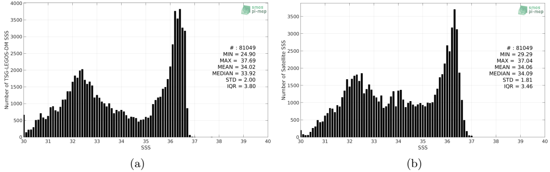
Figure 2: Histograms of SSS from TSG-LEGOS-DM (a) and SMOS-L3-CATDS-CECOS-LOCEAN-V3-18DAYS-25KM (b) considering all match-up pairs per bins of 0.1 over the Gulf Stream Pi-MEP region and for the full satellite product period.
