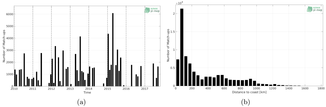
Figure 1: Number of match-ups between TSG-LEGOS-DM and SMOS-L3-CATDS-CECOS-LOCEAN-V3-18DAYS-25KM SSS as a function of time (a) and as function of the distance to coast (b) over the Gulf Stream Pi-MEP region and for the full satellite product period.
