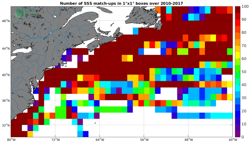
Figure 4: Number of SSS match-ups between TSG-LEGOS-DM SSS and the SMOS-L3-CATDS-CECOS-LOCEAN-V3-18DAYS-25KM SSS product for the Gulf Stream Pi-MEP region over 1°x1° boxes and for the full satellite product period.
