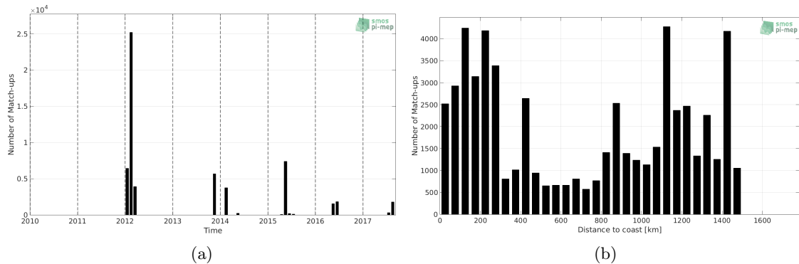
Figure 1: Number of match-ups between TSG-GOSUD-Sailing-ship and SMOS-L3-CATDS-CECOS-LOCEAN-V3-18DAYS-25KM SSS as a function of time (a) and as function of the distance to coast (b) over the Gulf Stream Pi-MEP region and for the full satellite product period.
