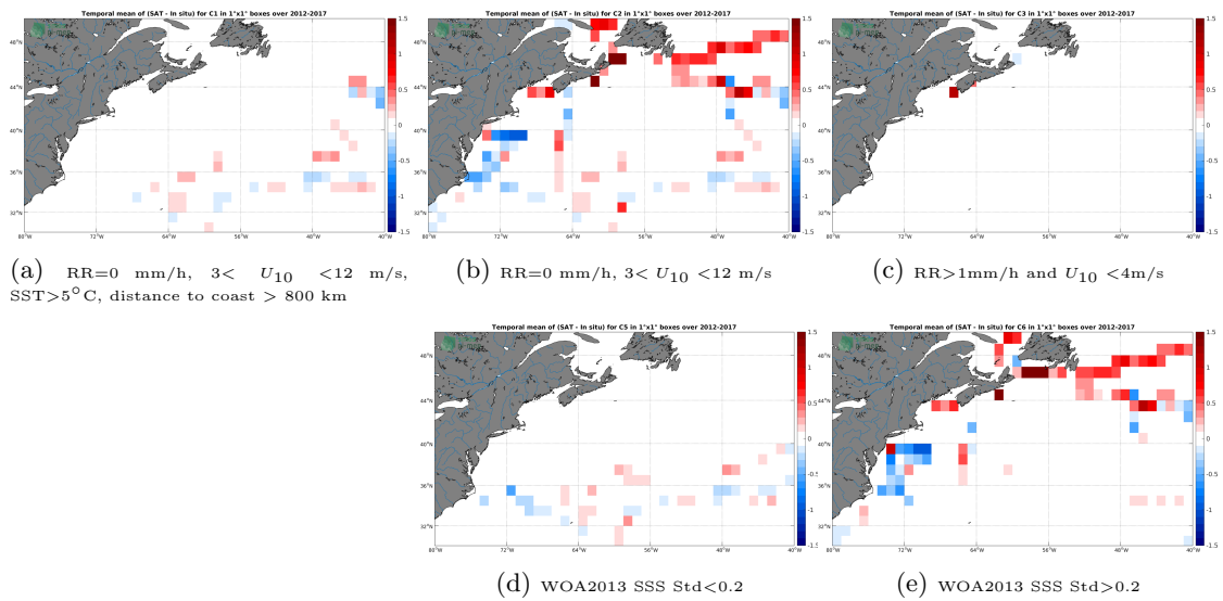
Figure 12: Temporal mean gridded over spatial boxes of size 1^\circ \times 1^\circ of \Delta SSS (SMOS-L3-CATDS-CECOS-LOCEAN-V3-18DAYS-25KM - TSG-GOSUD-Sailing-ship) for 5 different subdatasets corresponding to: RR=0 mm/h, 3 < U_{10} < 12 m/s, SST > 5°C, distance to coast > 800 km (a), RR=0 mm/h, 3 < U_{10} < 12 m/s (b), RR > 1mm/h and U_{10} < 4 m/s (c), WOA2013 SSS Std < 0.2 (d), WOA2013 SSS Std > 0.2 (e).
