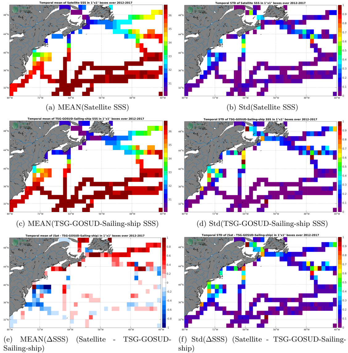
Figure 6: Temporal mean (left) and Std (right) of SSS from SMOS-L3-CATDS-CECOS-LOCEAN-V3-18DAYS-25KM (top), TSG-GOSUD-Sailing-ship (middle), and of \Delta SSS (Satellite - TSG-GOSUD-Sailing-ship). Only match-up pairs are used to generate these maps.
