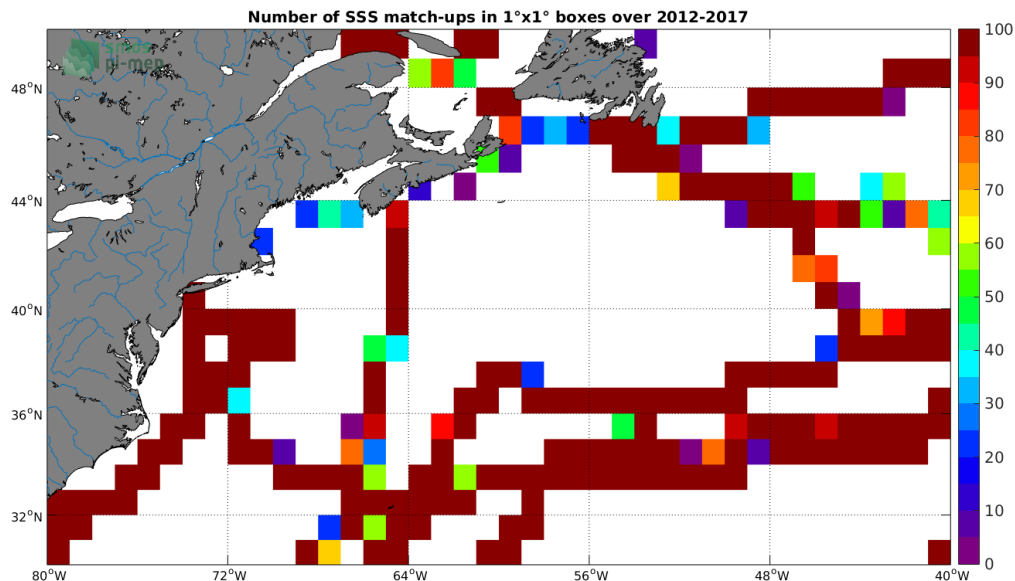
Figure 4: Number of SSS match-ups between TSG-GOSUD-Sailing-ship SSS and the SMOS-L3-CATDS-CECOS-LOCEAN-V3-18DAYS-25KM SSS product for the Gulf Stream Pi-MEP region over 1^\circ \times 1^\circ boxes and for the full satellite product period.
