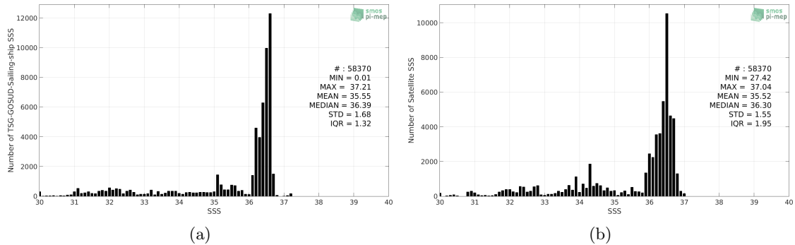
Figure 2: Histograms of SSS from TSG-GOSUD-Sailing-ship (a) and SMOS-L3-CATDS-CECOS-LOCEAN-V3-18DAYS-25KM (b) considering all match-up pairs per bins of 0.1 over the Gulf Stream Pi-MEP region and for the full satellite product period.
