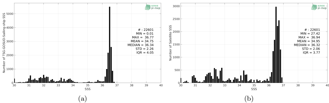
Figure 2: Histograms of SSS from TSG-GOSUD-Sailing-ship (a) and SMOS-L3-CATDS-CECOS-LOCEAN-V3-18DAYS-25KM (b) considering all match-up pairs per bins of 0.1 over the Gulf Stream Pi-MEP region and for the full satellite product period.
