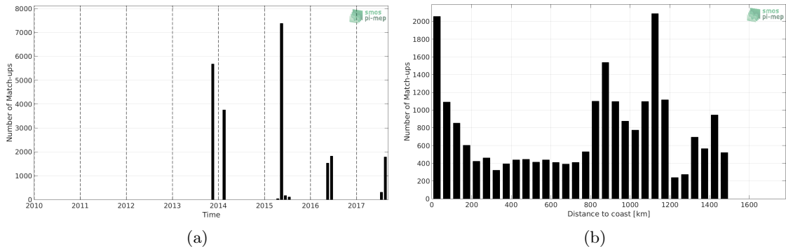
Figure 1: Number of match-ups between TSG-GOSUD-Sailing-ship and SMOS-L3-CATDS-CECOS-LOCEAN-V3-18DAYS-25KM SSS as a function of time (a) and as function of the distance to coast (b) over the Gulf Stream Pi-MEP region and for the full satellite product period.
